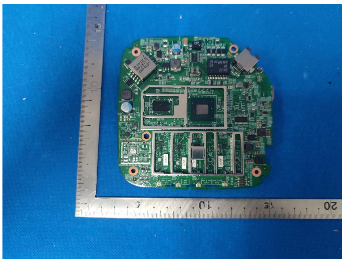
(2) EUT Photo(AP305C)
