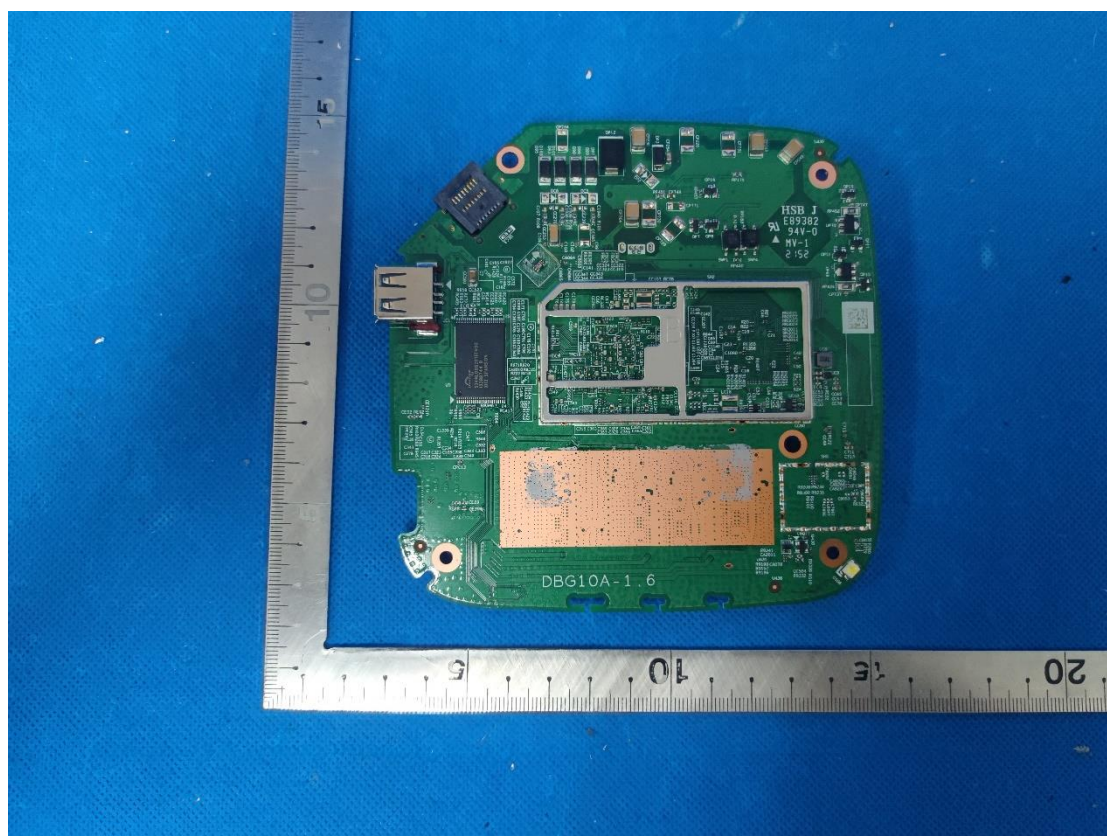
(2) EUT Photo(AP305C)
