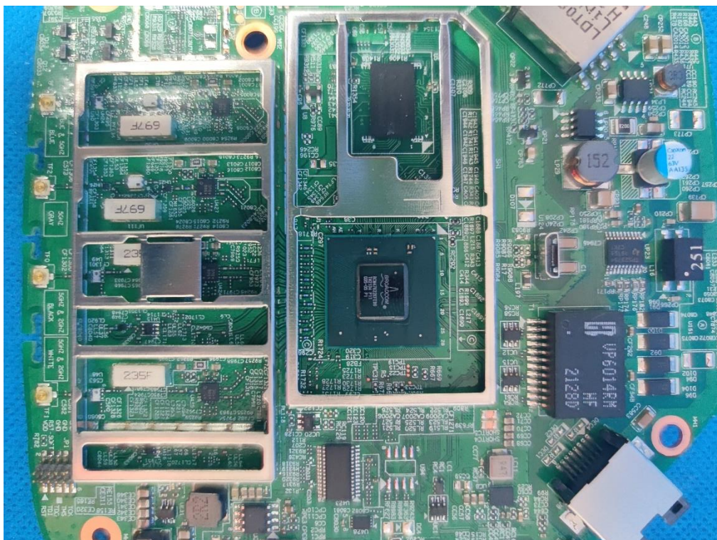
(4) EUT Photo(AP305C)
