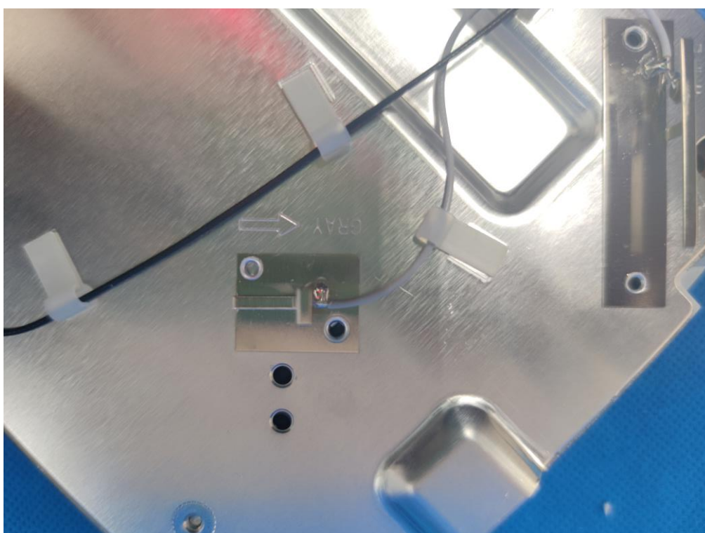
(8) EUT Photo(AP305C)
