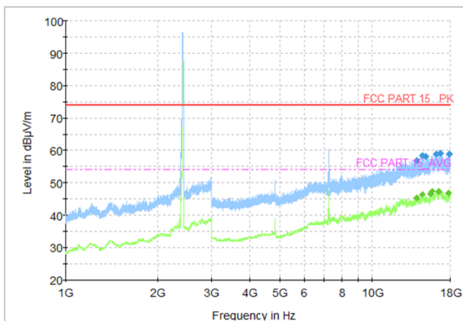
Fig.44 Radiated Spurious Emission (802.11n HT20, CH1, 1 GHz-18 GHz)
