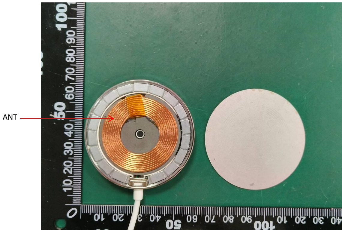
Internal Photo FCC ID: 2BFEUY103
