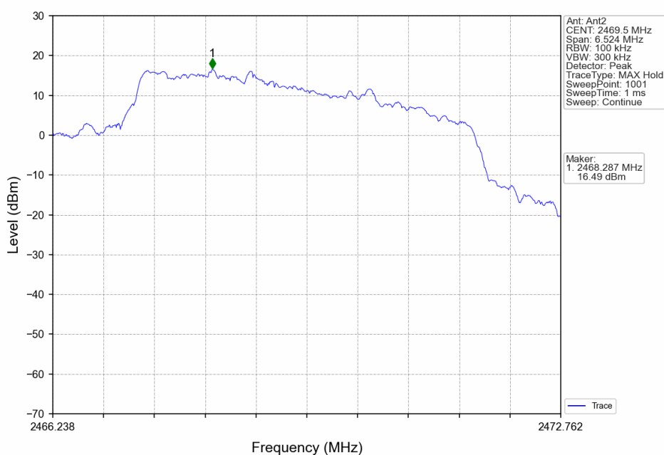
5M_HCH_2469.5MHz_Ant2_NTNV
