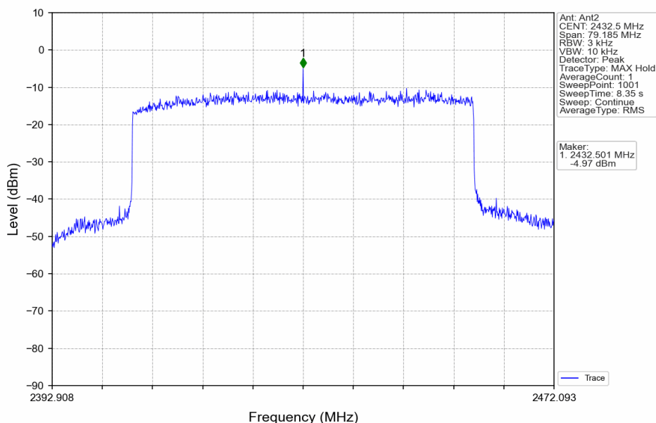
60M_LCH_2432.5MHz_Ant2_NTNV
