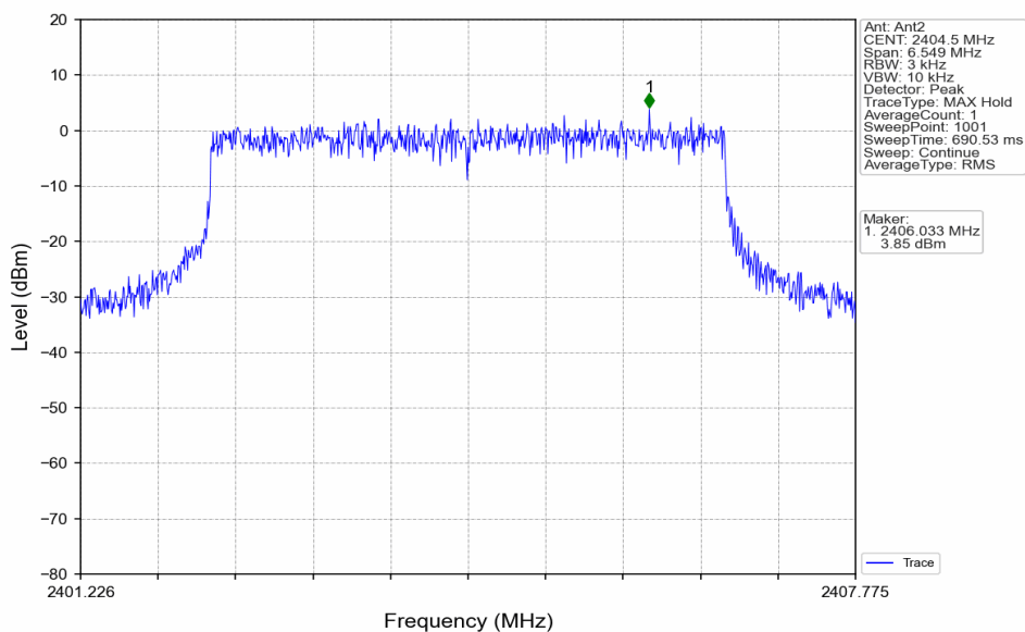
5M_LCH_2404.5MHz_Ant2_NTNV
