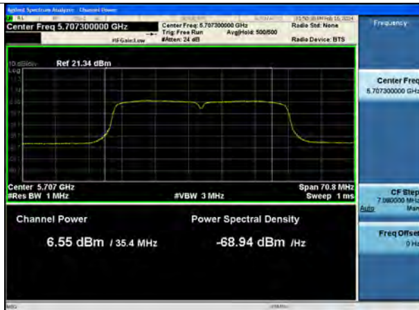
802.11n(HT40) UNII 2C Band
