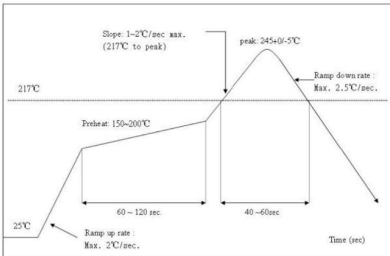
Figure 7-3 Oven temperature curve
