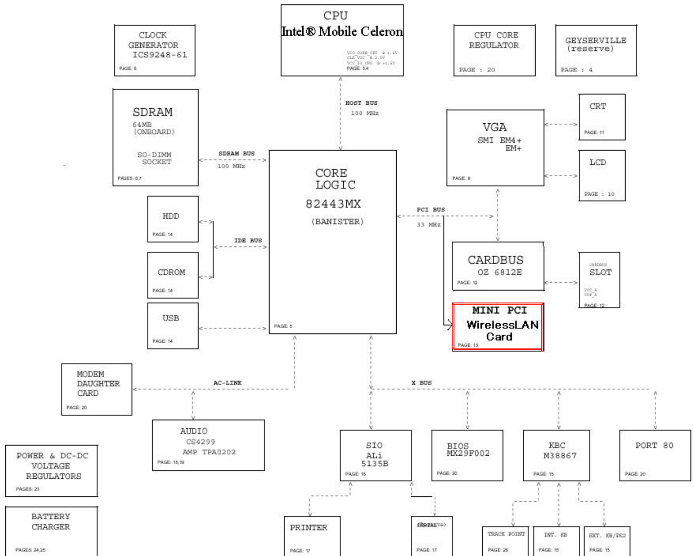
Figure 14 Block diagram of ThinkPad i 1300 and ThinkPad 130
