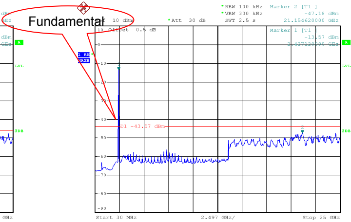
Mode: TX 11 n HT40 channel 6
