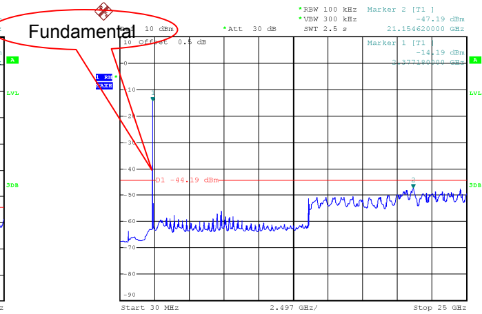
Mode: TX 11 n HT20 channel 6
