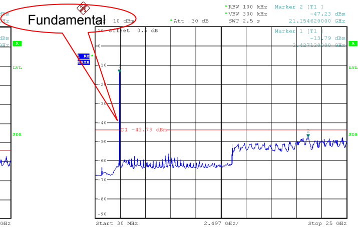
Mode: TX 11g channel 6
