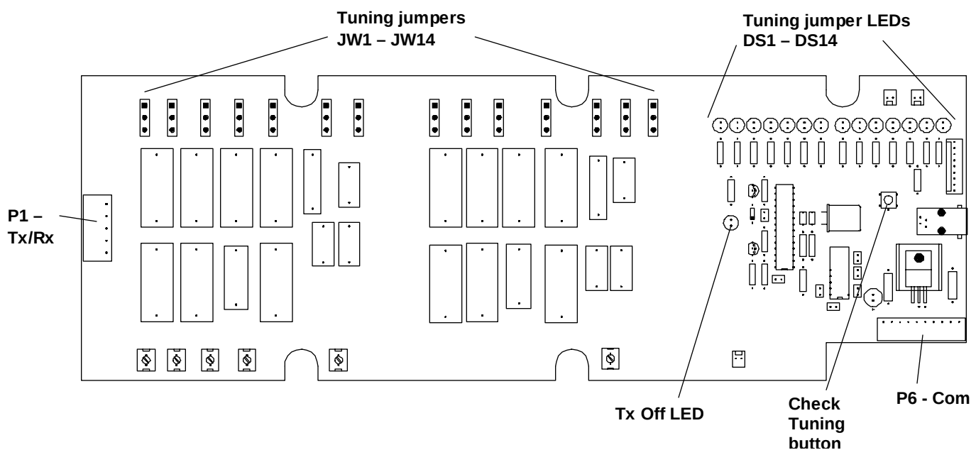
Figure 7. Capacitor board 0301-1532-01
