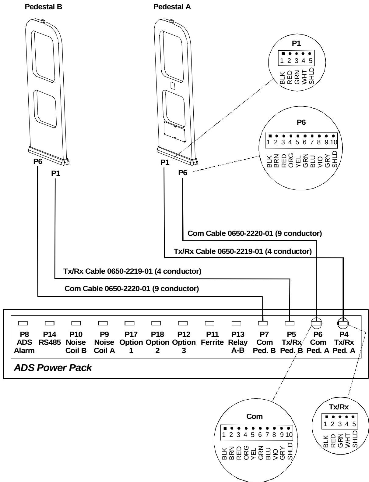
Figure 2. Wiring diagram
