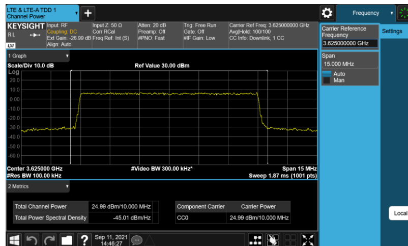
Band48-10MHz-256QAM-56690-E-TM3.1A-10
