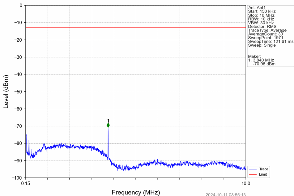
Band4_RMC_LCH_1712.4MHz_12.2kbps_RMC_NTNV
