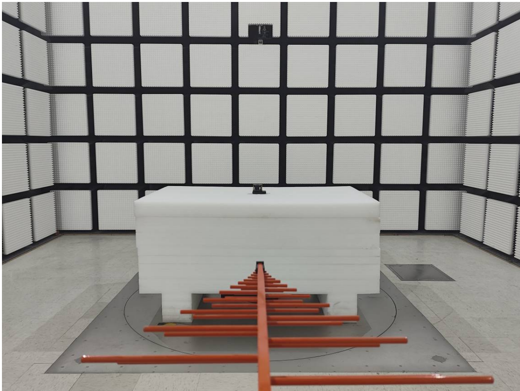
Radiated Emission 30M-1GHz View-M3
