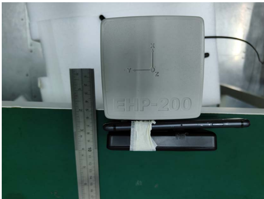
H-Field Position F Test distance 0-4cm M3
