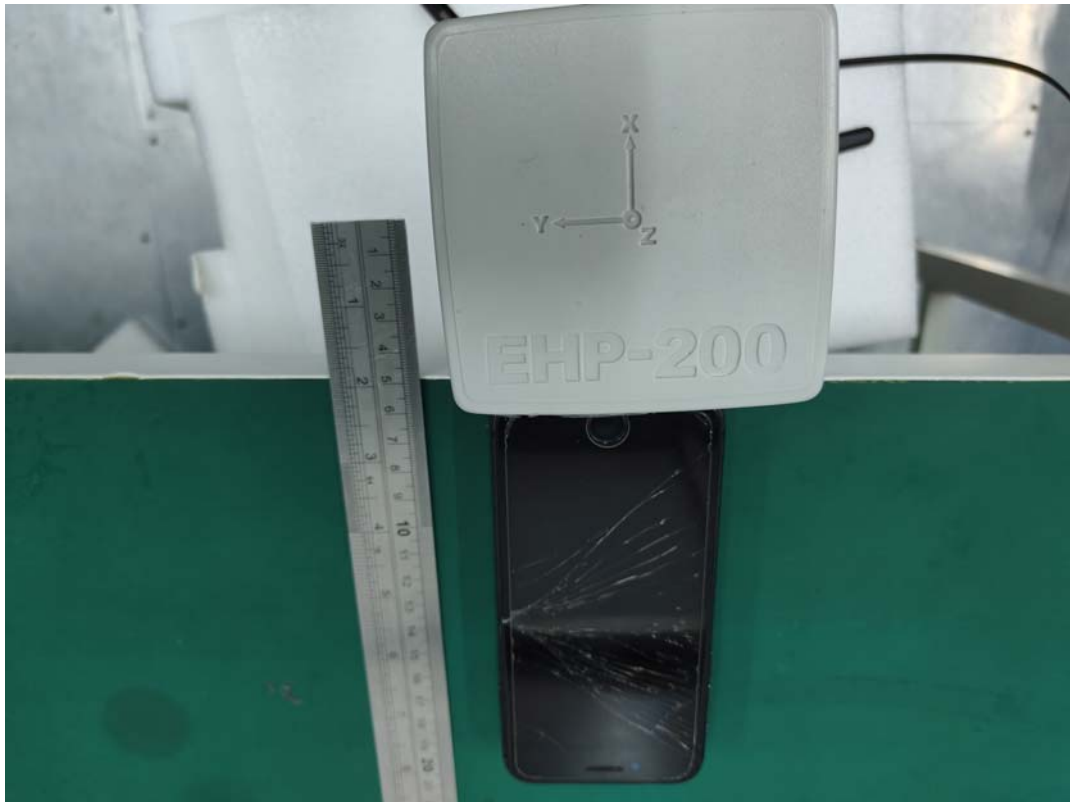
H-Field Position B Test distance 0-4cm M3
