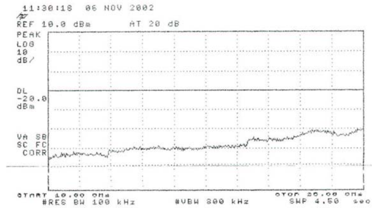
Figure 6.5 Antenna Conducted Spurious Emissions. (all channels)
