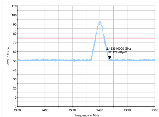
3DH5-Channel 78: Peak
