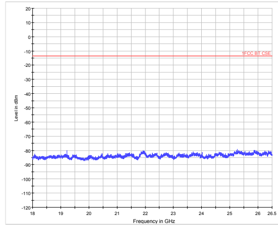
EDR-CH39 18GHz to 26.5GHz
