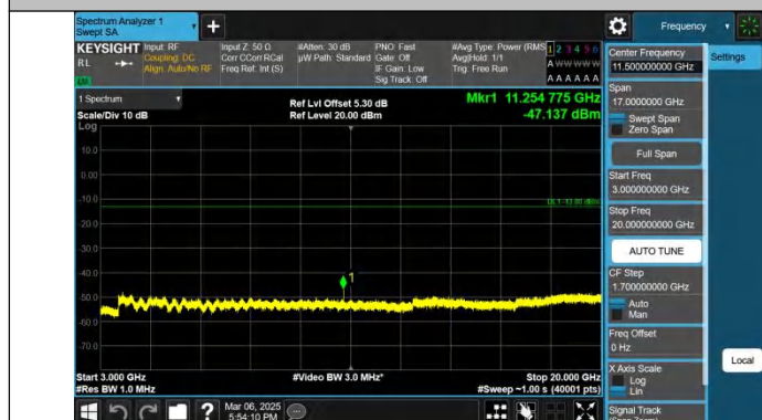
Band25-15MHz-QPSK-26365-1RB#0-3000~20000-PASS
