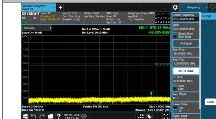
Band25-15MHz-QPSK-26365-1RB#0-30~1000-PASS
