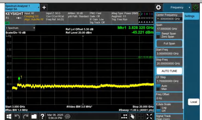
Band25-15MHz-QPSK-26615-1RB#74-3000~20000-PASS
