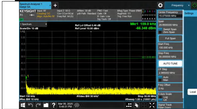
Band25-10MHz-QPSK-26090-1RB#49-0.15~30-PASS
