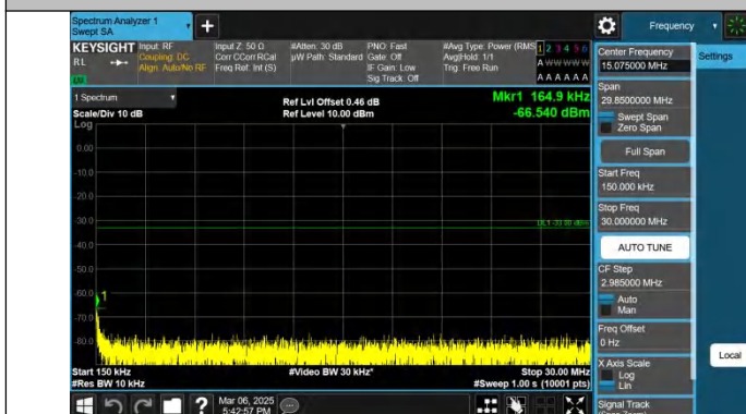
Band25-5MHz-QPSK-26665-1RB#24-0.15~30-PASS
