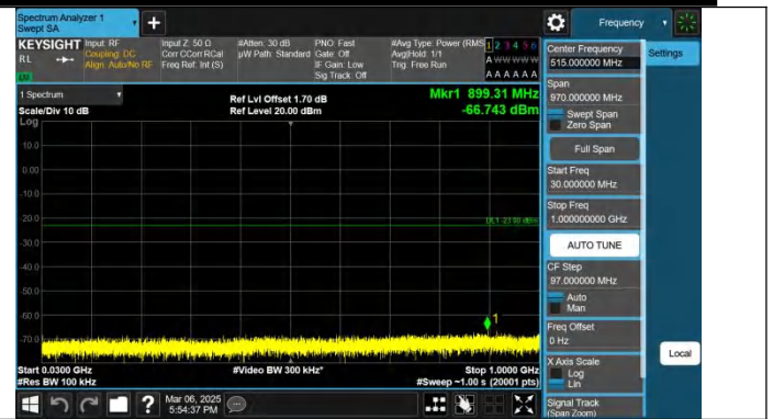
Band25-15MHz-QPSK-26365-1RB#74-30~1000-PASS
