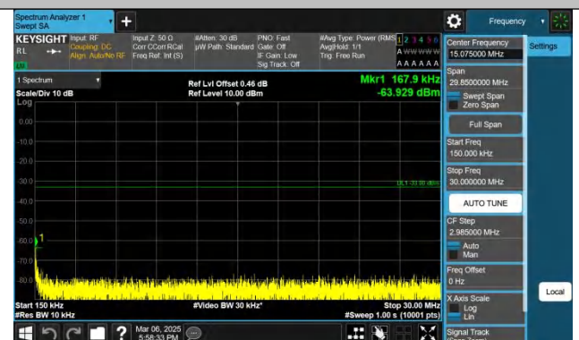
Band25-20MHz-QPSK-26140-1RB#0-0.15~30-PASS
