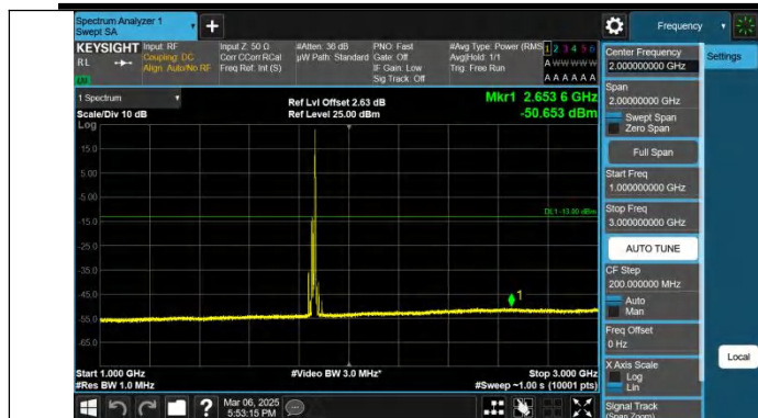
Band25-15MHz-QPSK-26115-1RB#74-1000~3000-PASS
