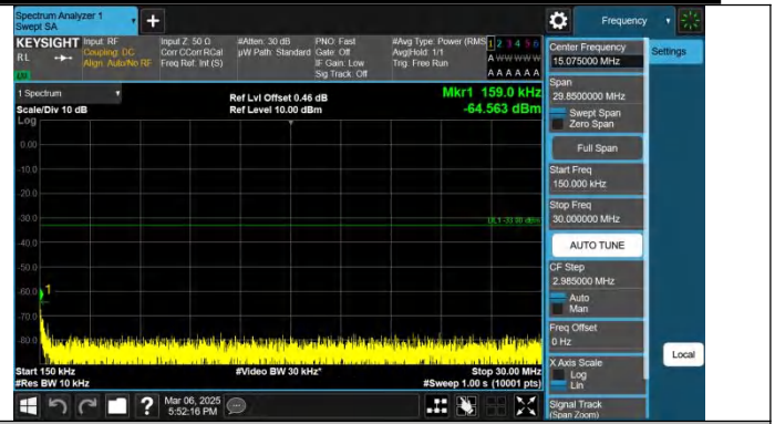
Band25-15MHz-QPSK-26115-1RB#0-0.15~30-PASS
