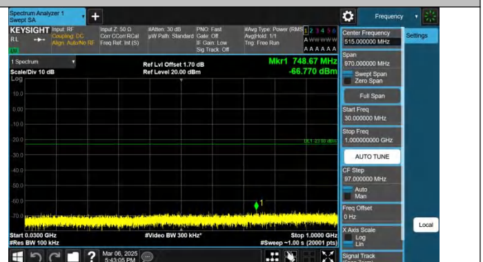
Band25-5MHz-QPSK-26665-1RB#24-30~1000-PASS
