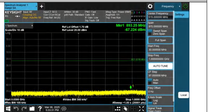
Band25-3MHz-QPSK-26055-1RB#14-30~1000-PASS
