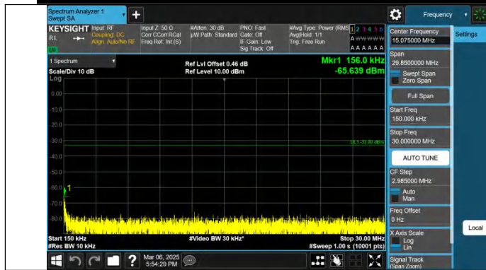
Band25-15MHz-QPSK-26365-1RB#74-0.15~30-PASS
