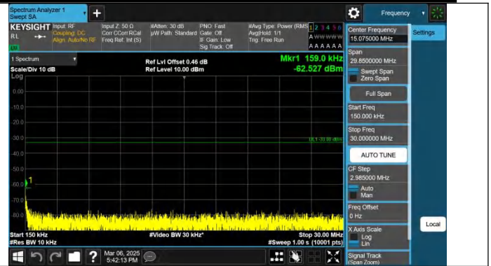
Band25-5MHz-QPSK-26665-1RB#0-0.15~30-PASS
