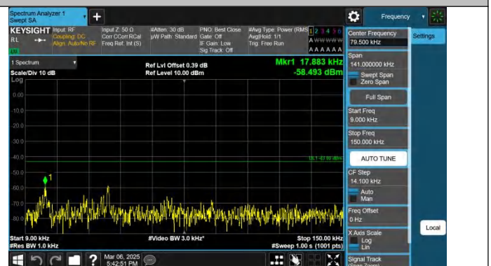
Band25-5MHz-QPSK-26665-1RB#24-0.009~0.15-PASS
