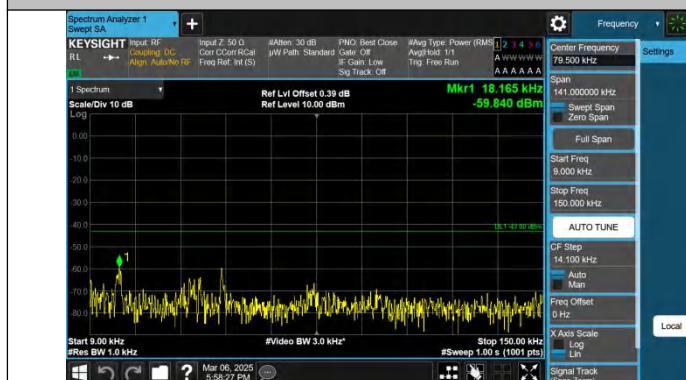
Band25-20MHz-QPSK-26140-1RB#0-0.009~0.15-PASS
