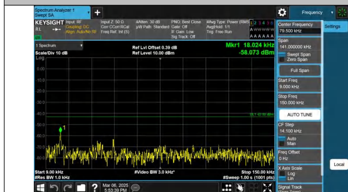
Band25-15MHz-QPSK-26365-1RB#0-0.009~0.15-PASS
