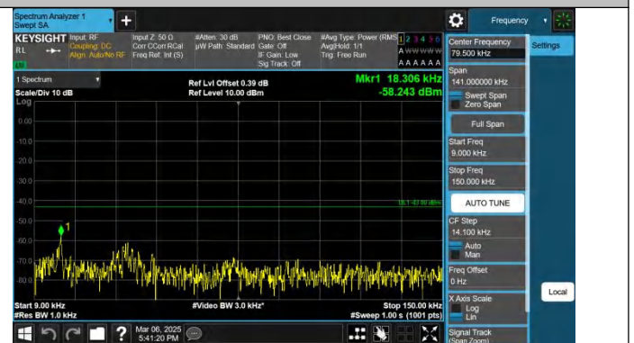
Band25-5MHz-QPSK-26365-1RB#24-0.009~0.15-PASS
