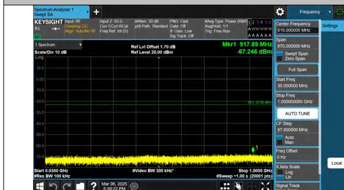
Band25-5MHz-QPSK-26065-1RB#0-30~1000-PASS
