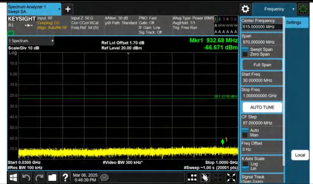
Band25-10MHz-QPSK-26090-1RB#49-30~1000-PASS
