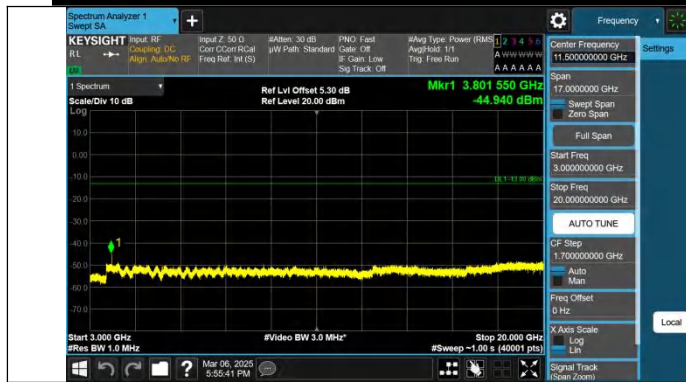
Band25-15MHz-QPSK-26615-1RB#0-3000~20000-PASS
