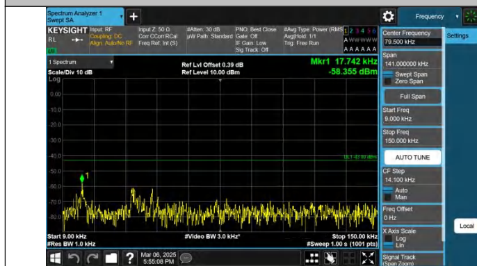
Band25-15MHz-QPSK-26615-1RB#0-0.009~0.15-PASS
