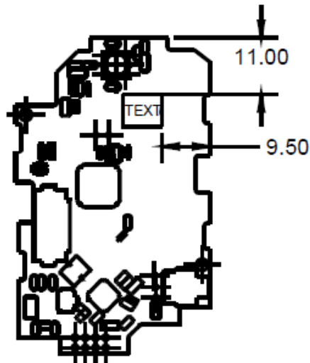
COMPLIANCE LABEL LOCATION BACK VIEW OF B8200
