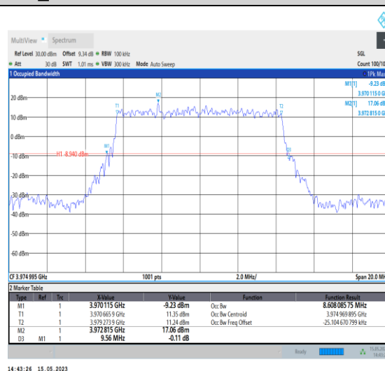
1-N77-3700-3980-PC1-30-10-H-2-DFT-PI2BPSK-Out ter Full-24@0-Ant0-8.608-9.560-≤10-PASS
