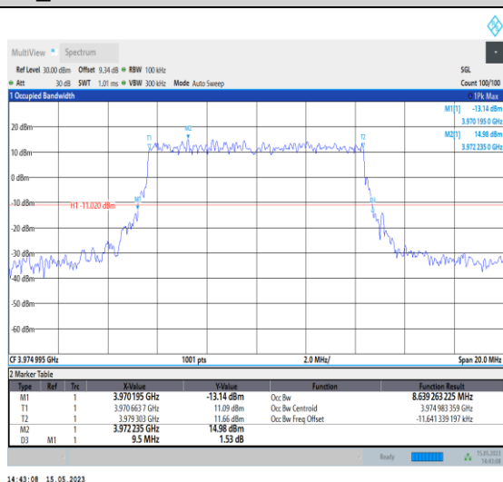
1-N77-3700-3980-PC1-30-10-H-1-DFT-QPSK-Outer_ Full-24@0-Ant0-8.639-9.500-≤10-PASS
