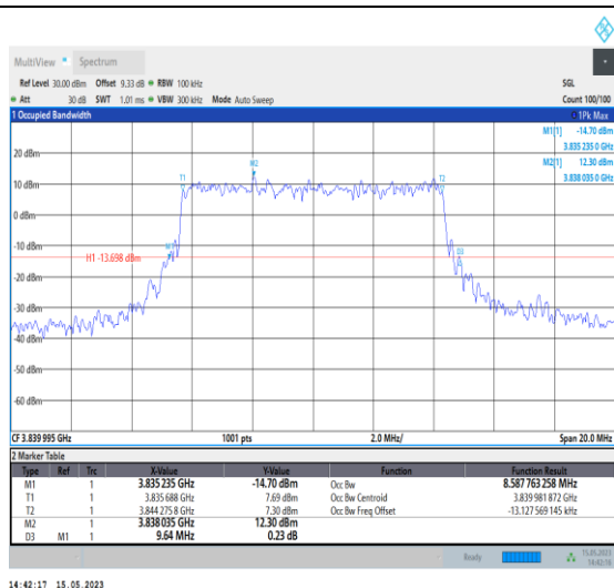
1-N77-3700-3980-PC1-30-10-M-8-CP-64QAM-Outer Full-24@0-Ant0-8.588-9.640-≤10-PASS
