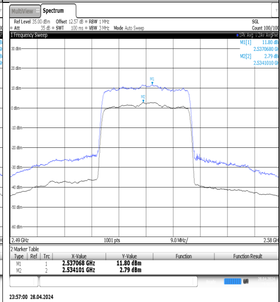
NTNV-N7-PC3-15-30-M-DFT-16QAM-Outter_Full-Ant1-PASS
