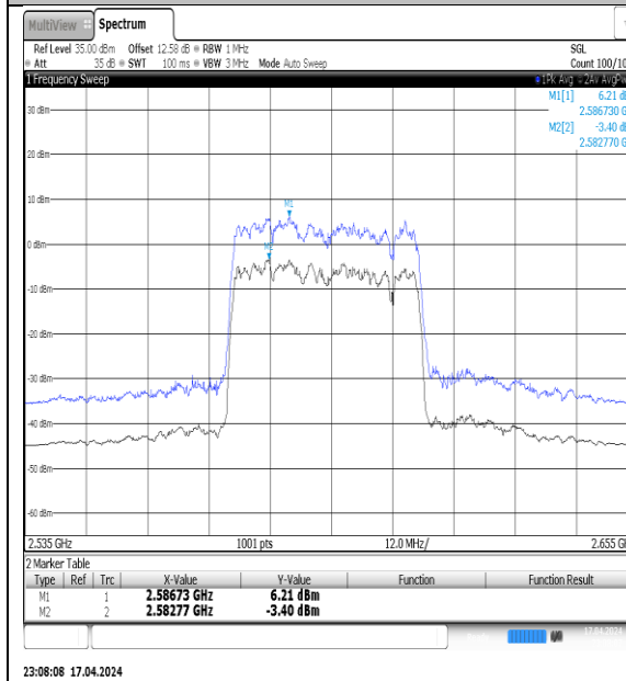
NTNV-N38-PC3-30-40-M-DFT-16QAM-Outer_Full-Ant1-PASS
