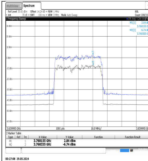
NTNV-N78-3700-3800-PC3-30-60-M-DFT- 16QAM-Outer_Full-Ant1-PASS
