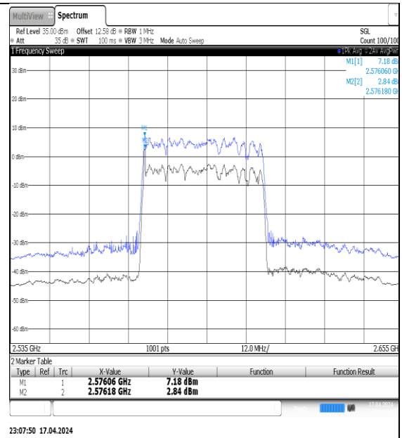
NTNV-N38-PC3-30-40-M-DFT-QPSK-Outer_Full-Ant1-PASS
