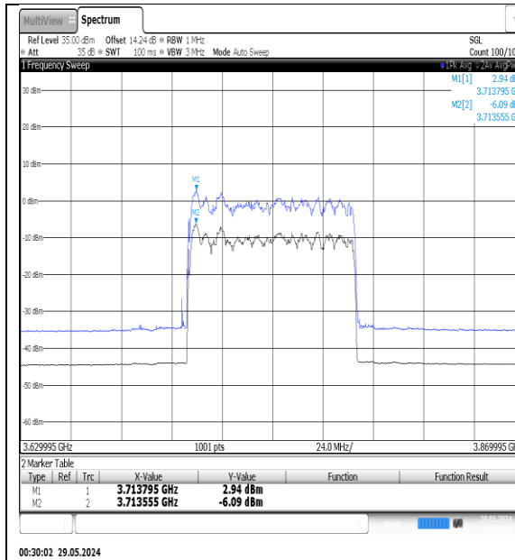
NTNV-N78-3700-3800-PC3-30-80-M-DFT- 16QAM-Outer_Full-Ant1-PASS
