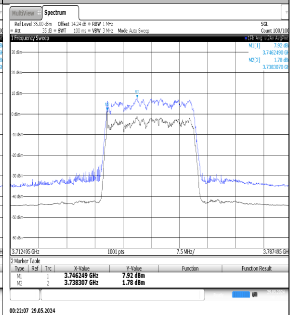
NTNV-N78-3700-3800-PC3-30-25-M-DFT-QPSK- Outer_Full-Ant1-PASS
