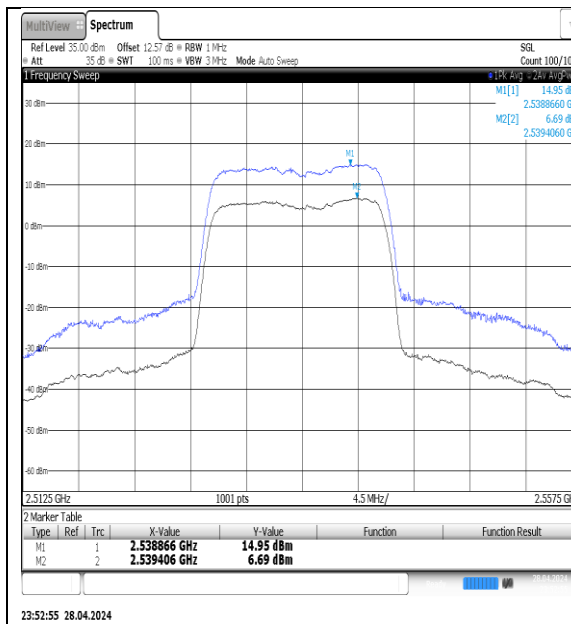
NTNV-N7-PC3-15-15-M-DFT-QPSK-Outet_Full-Ant1-PASS
