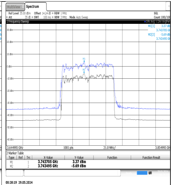
NTNV-N78-3700-3800-PC3-30-70-M-DFT-QPSK- Outer_Full-Ant1-PASS
