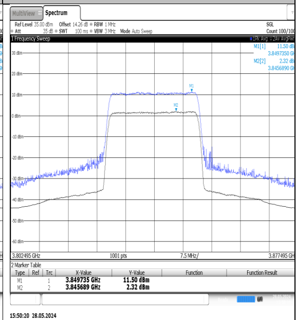
NTNV-N77-3700-3980-PC3-30-25-M-DFT-QPSK- Outer_Full-Ant1-PASS
