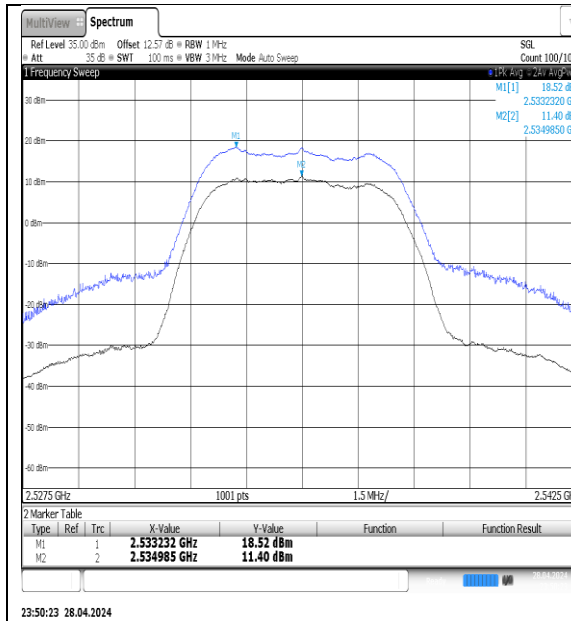
NTNV-N7-PC3-15-5-M-DFT-QPSK-Outer_Full- Ant1-PASS
