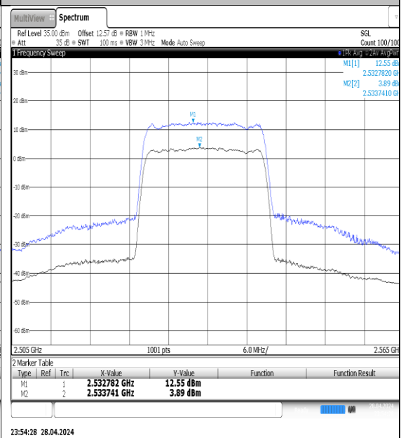
NTNV-N7-PC3-15-20-M-DFT-16QAM-Outet_Full-Ant1-PASS
