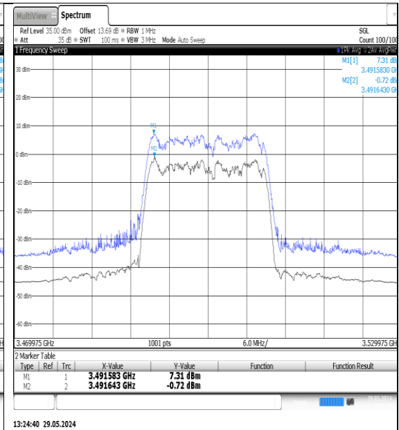
NTNV-N77-3450-3550-PC3-30-20-M-DFT-QPSK- Outer_Full-Ant1-PASS
