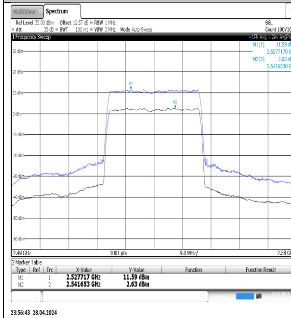
NTNV-N7-PC3-15-30-M-DFT-QPSK-Outter_Full-Ant1-PASS
