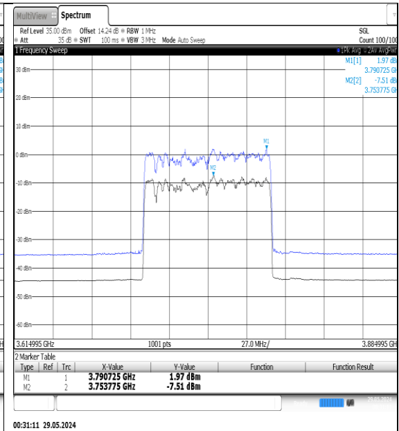
NTNV-N78-3700-3800-PC3-30-90-M-DFT-QPSK- Outer_Full-Ant1-PASS
