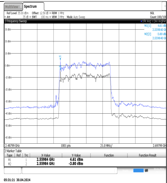
NTNV-N41-PC3-30-70-M-DFT-QPSK-Outer_Full-Ant1-PASS
