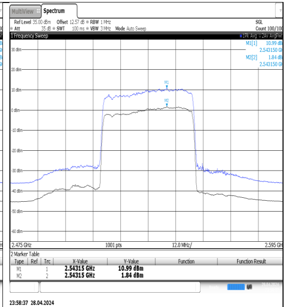
NTNV-N7-PC3-15-40-M-DFT-16QAM-Outter_Full-Ant1-PASS
