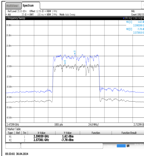
NTNV-N41-PC3-30-80-M-DFT-16QAM-Outer_Full-Ant1-PASS
