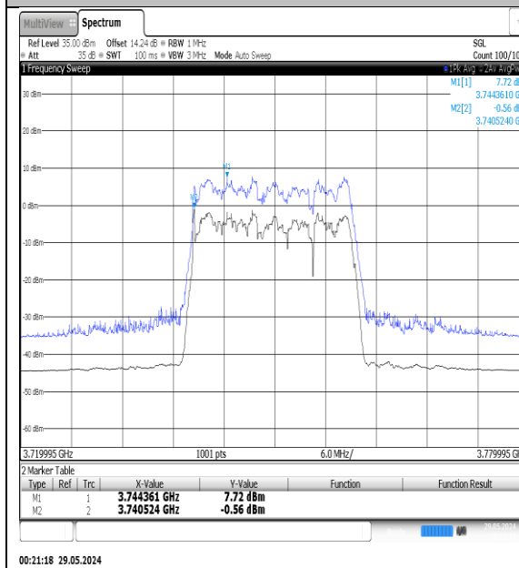
NTNV-N78-3700-3800-PC3-30-20-M-DFT- 16QAM-Outer_Full-Ant1-PASS
