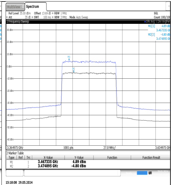
NTNV-N77-3450-3550-PC3-30-90-M-DFT-QPSK- Outer_Full-Ant1-PASS
