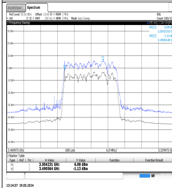
NTNV-N77-3450-3550-PC3-30-20-M-DFT- 16QAM-Outer_Full-Ant1-PASS
