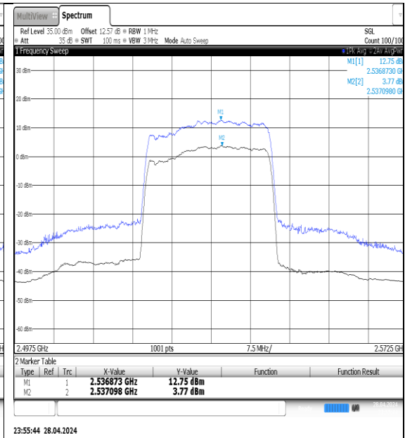
NTNV-N7-PC3-15-25-M-DFT-16QAM-Outter_Full-Ant1-PASS
