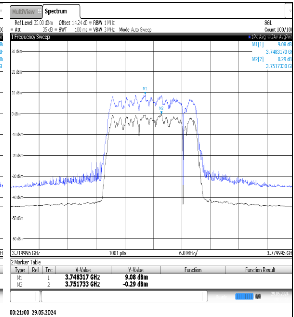
NTNV-N78-3700-3800-PC3-30-20-M-DFT-QPSK- Outer_Full-Ant1-PASS
