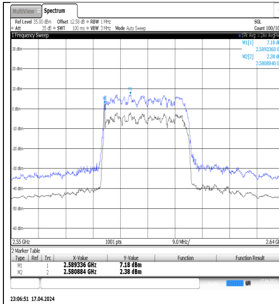
NTNV-N38-PC3-30-30-M-DFT-16QAM-Outer_Full-Ant1-PASS
