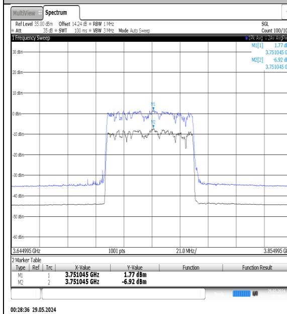
NTNV-N78-3700-3800-PC3-30-70-M-DFT- 16QAM-Outer_Full-Ant1-PASS
