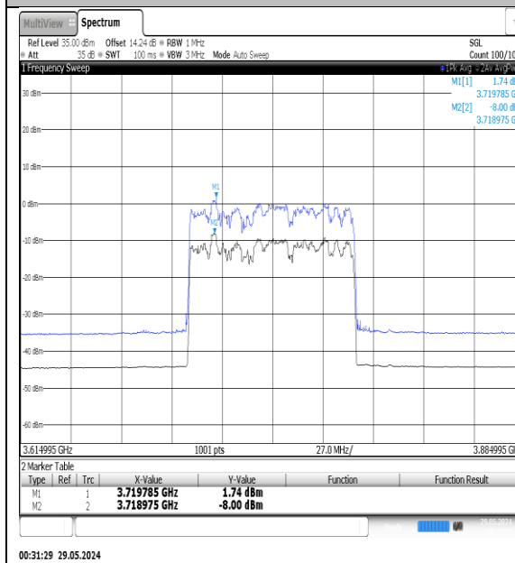
NTNV-N78-3700-3800-PC3-30-90-M-DFT- 16QAM-Outer_Full-Ant1-PASS
