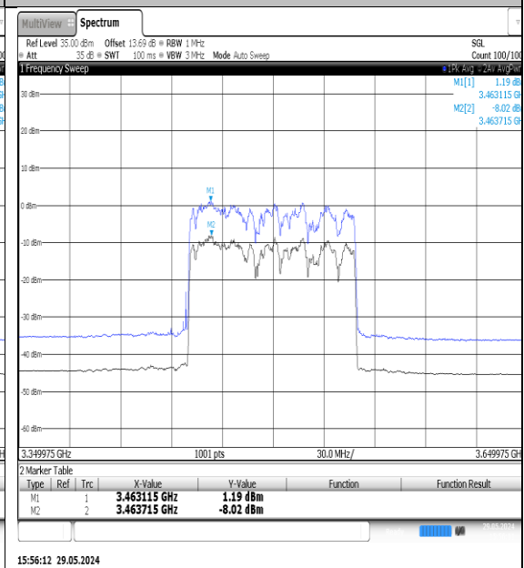
NTNV-N77-3450-3550-PC3-30-100-M-DFT- QPSK-Outer_Full-Ant1-PASS
