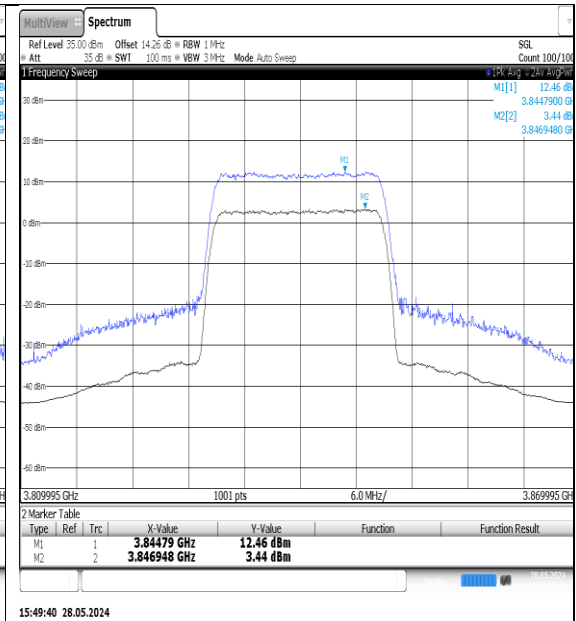
NTNV-N77-3700-3980-PC3-30-20-M-DFT-QPSK- Outer_Full-Ant1-PASS
