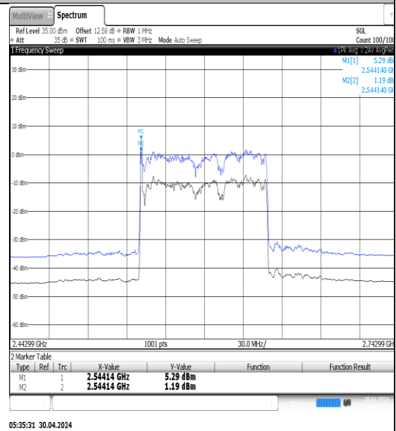
NTNV-N41-PC3-30-100-M-DFT-QPSK-Outer_Full-Ant1-PASS
