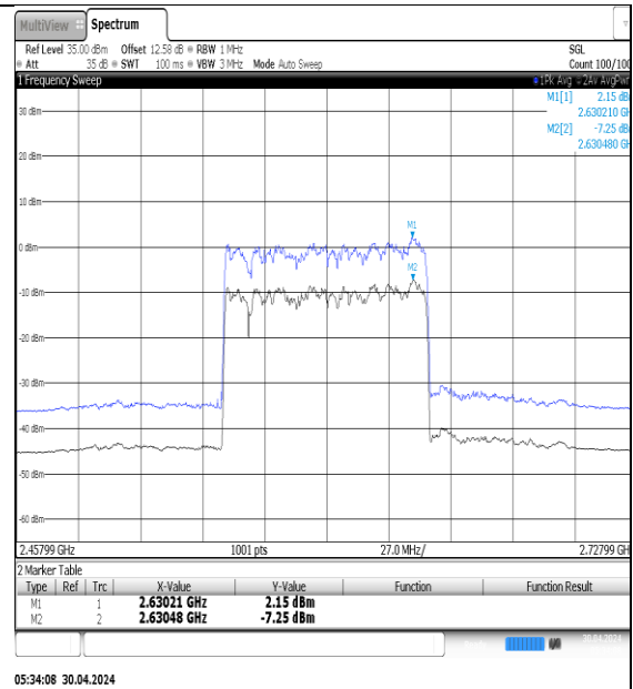
NTNV-N41-PC3-30-90-M-DFT-QPSK-Outer_Full-Ant1-PASS
