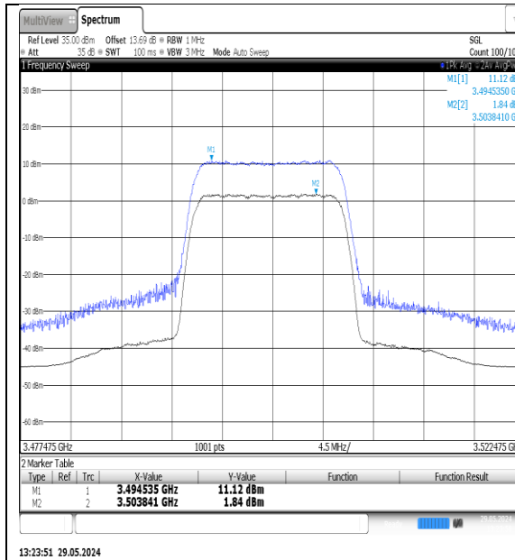
NTNV-N77-3450-3550-PC3-30-15-M-DFT- 16QAM-Outer_Full-Ant1-PASS
