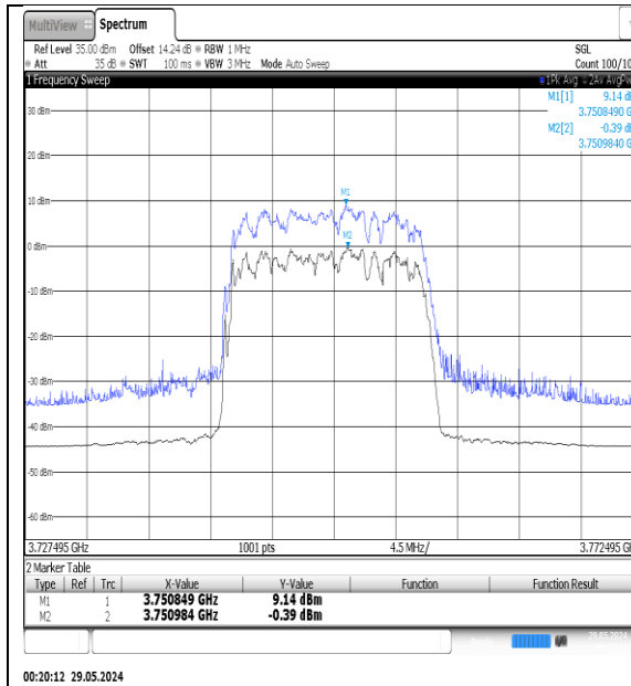
NTNV-N78-3700-3800-PC3-30-15-M-DFT- 16QAM-Outer_Full-Ant1-PASS
