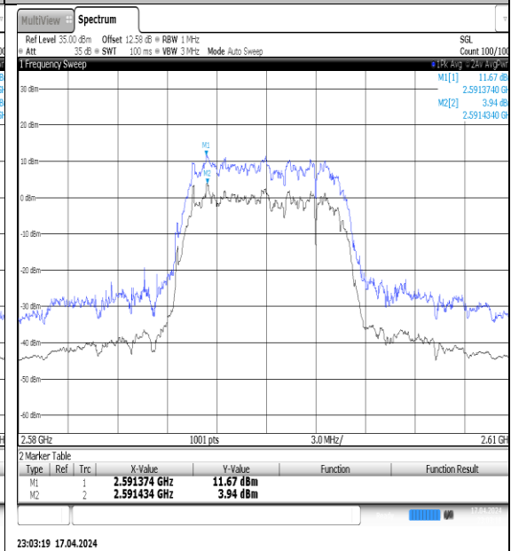
NTNV-N38-PC3-30-10-M-DFT-16QAM-Outter_Full-Ant1-PASS
