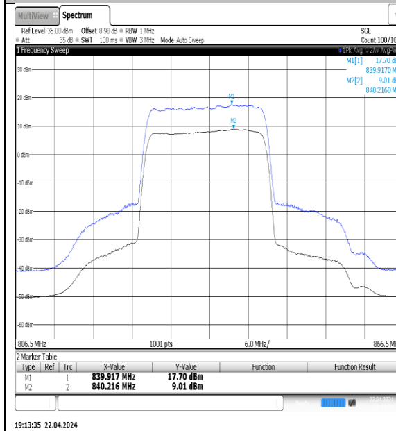
NTNV-N5-PC3-15-20-M-DFT-QPSK-Outet_Full-Ant1-PASS
