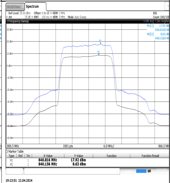
NTNV-N5-PC3-15-20-M-DFT-16QAM-Outet_Full-Ant1-PASS
