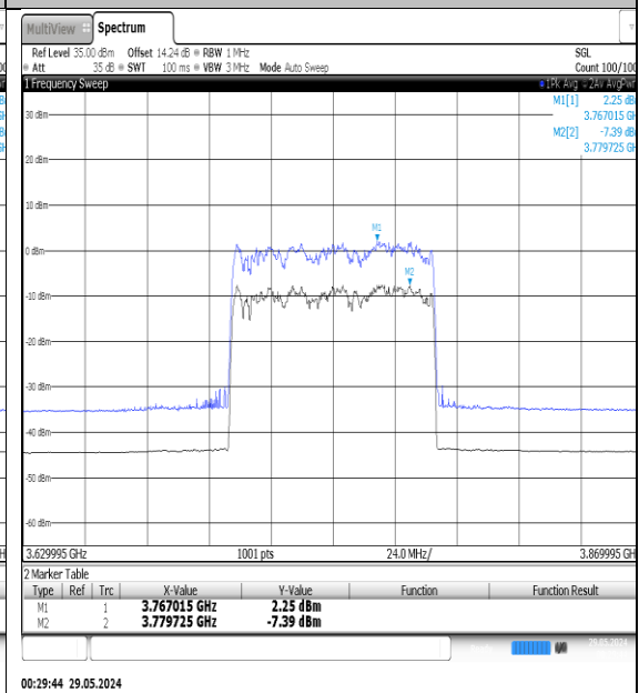
NTNV-N78-3700-3800-PC3-30-80-M-DFT-QPSK- Outer_Full-Ant1-PASS
