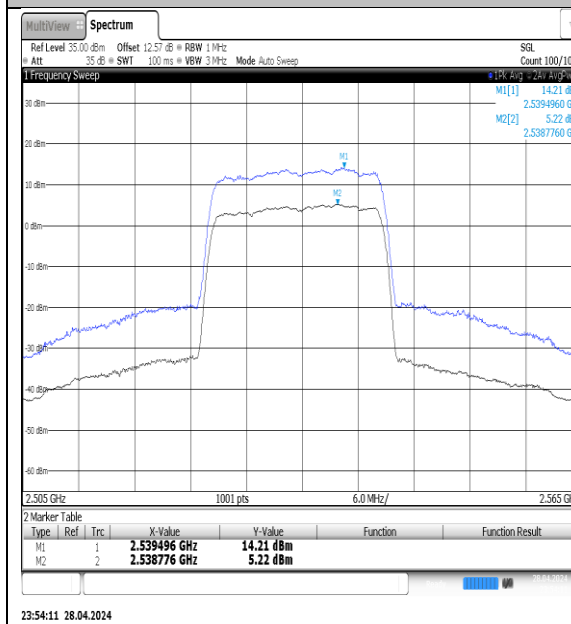
NTNV-N7-PC3-15-20-M-DFT-QPSK-Outet_Full-Ant1-PASS
