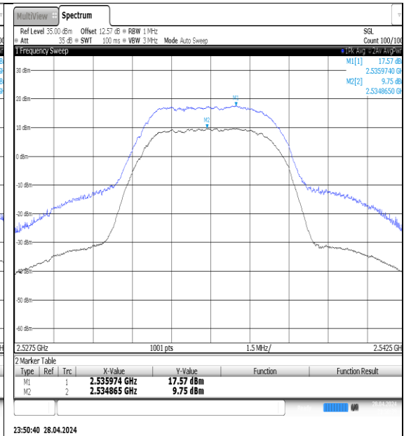
NTNV-N7-PC3-15-5-M-DFT-16QAM-Outer_Full- Ant1-PASS
