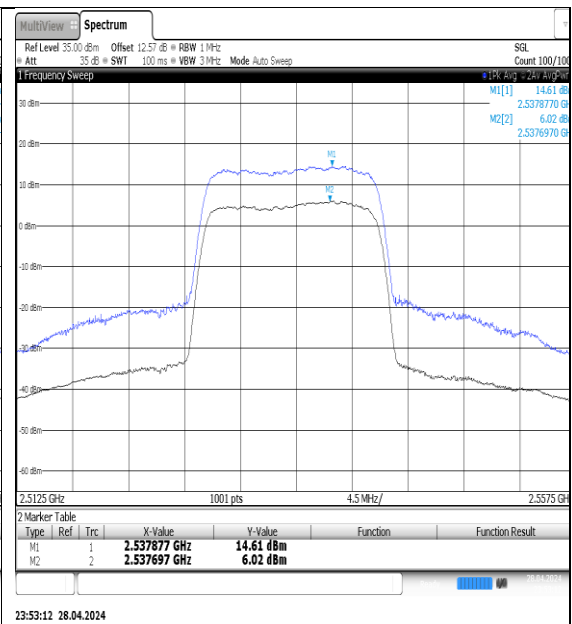
NTNV-N7-PC3-15-15-M-DFT-16QAM-Outet_Full-Ant1-PASS
