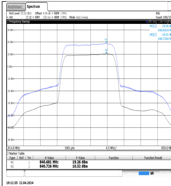
NTNV-N5-PC3-15-15-M-DFT-QPSK-Outet_Full-Ant1-PASS
