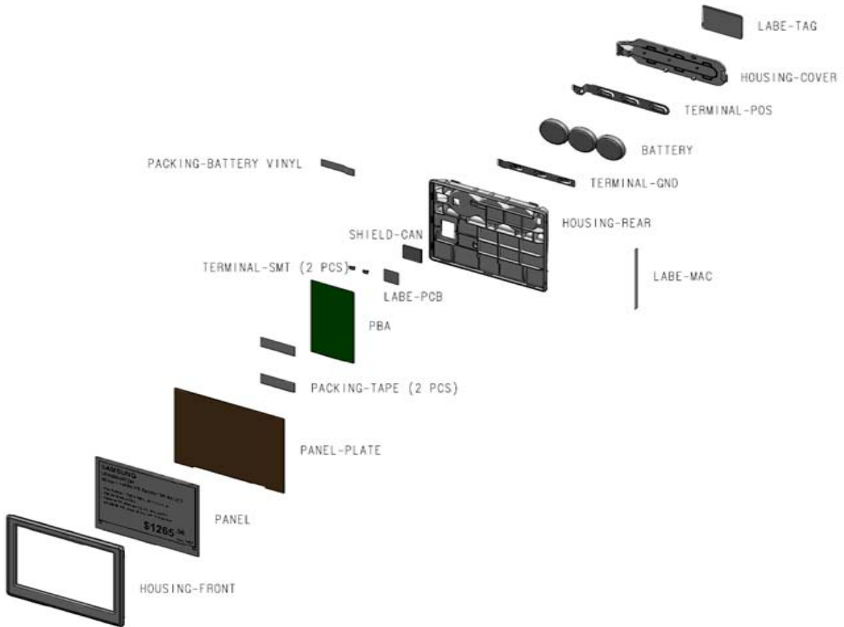
Figure 4Exploded View
