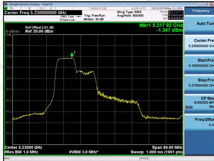
11AX40SISO-Ant1-5230-106Tone-RU53-PASS
