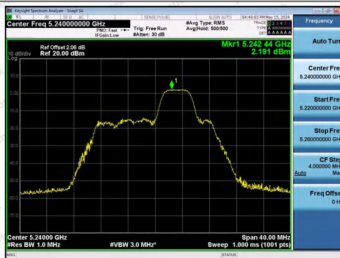
11AX20SISO-Ant1-5240-52Tone-RU39-PASS
