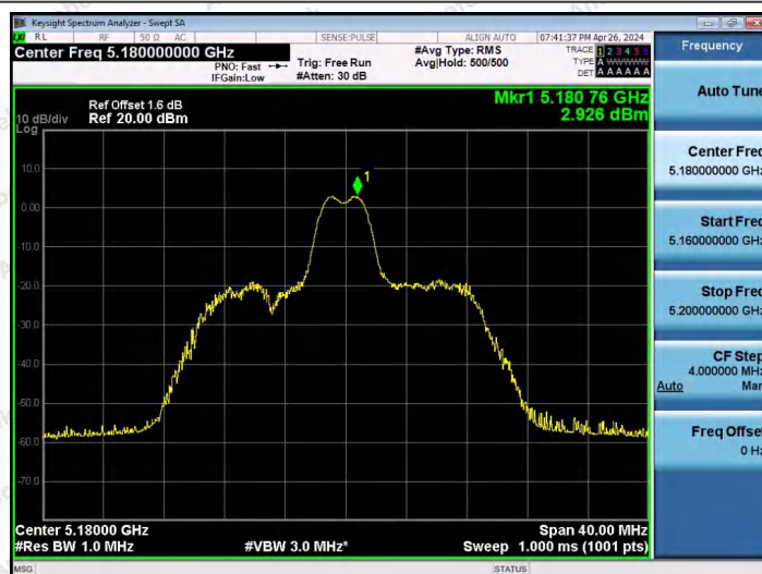
11AX20SISO-Ant1-5180-26Tone-RU4-PASS
