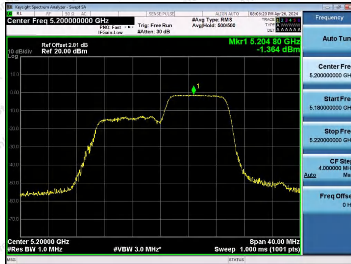
11AX20SISO-Ant1-5200-106Tone-RU54-PASS
