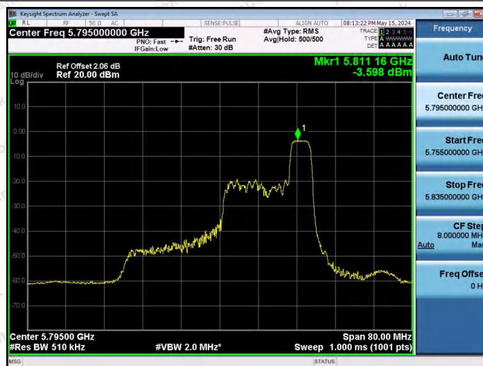
11AX40SISO-Ant1-5795-52Tone-RU44-PASS
