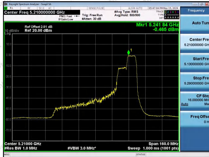
11AX80SISO-Ant1-5210-106Tone-RU60-PASS
