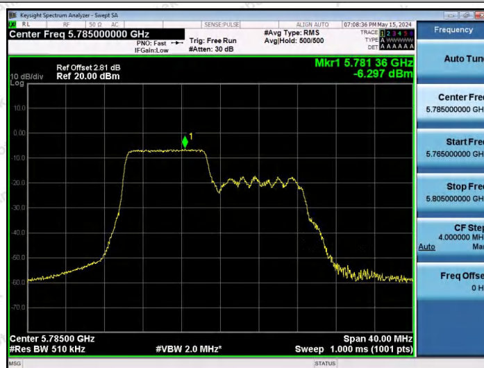
11AX20SISO-Ant1-5785-106Tone-RU53-PASS
