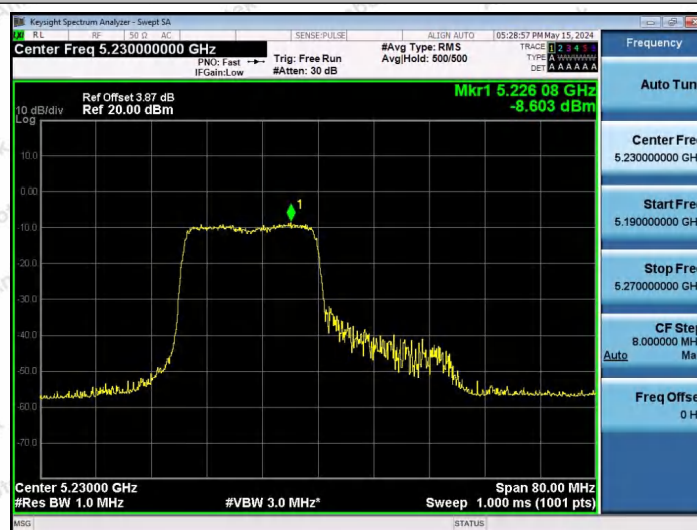
11AX40SISO-Ant1-5230-242Tone-RU61-PASS
