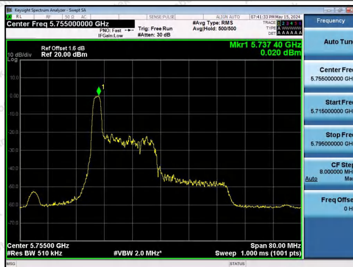
11AX40SISO-Ant1-5755-26Tone-RU0-PASS
