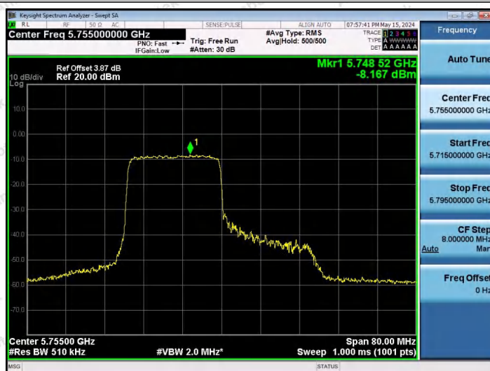
11AX40SISO-Ant1-5755-242Tone-RU61-PASS
