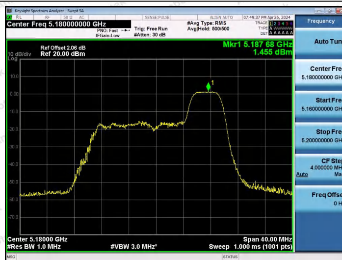
11AX20SISO-Ant1-5180-52Tone-RU40-PASS
