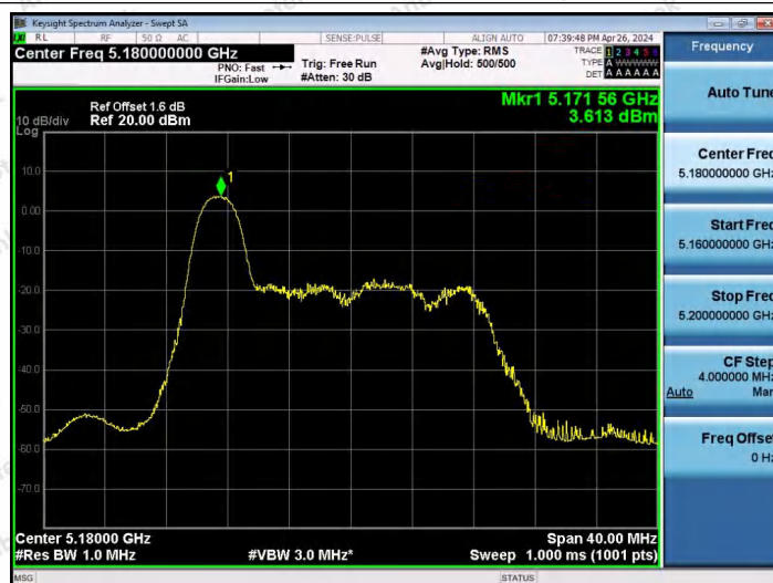
11AX20SISO-Ant1-5180-26Tone-RU0-PASS
