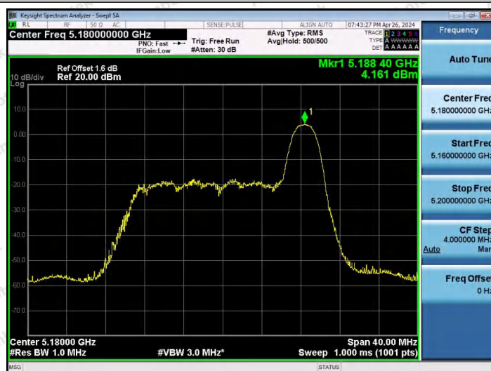
11AX20SISO-Ant1-5180-26Tone-RU8-PASS
