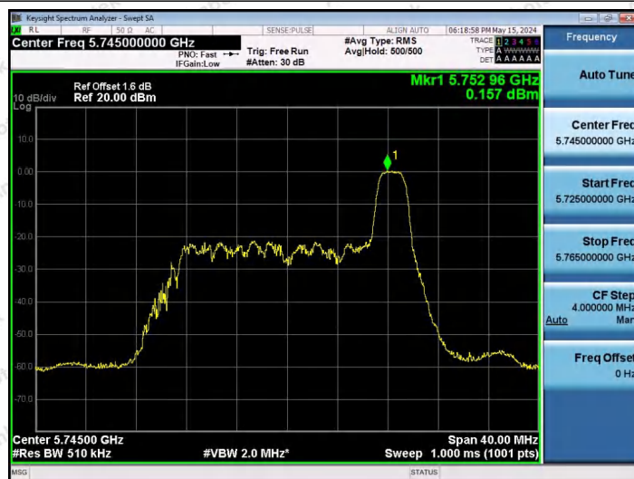
11AX20SISO-Ant1-5745-26Tone-RU8-PASS
