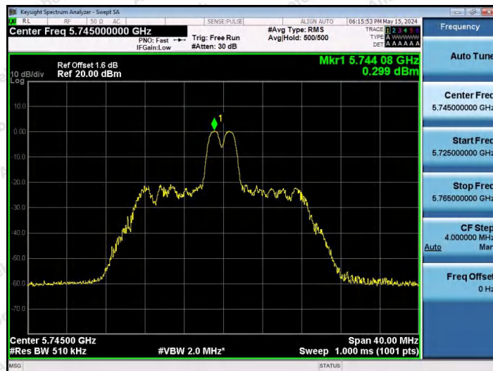
11AX20SISO-Ant1-5745-26Tone-RU4-PASS
