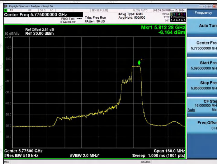
11AX80SISO-Ant1-5775-106Tone-RU60-PASS
