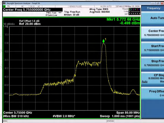
11AX40SISO-Ant1-5755-26Tone-RU17-PASS
