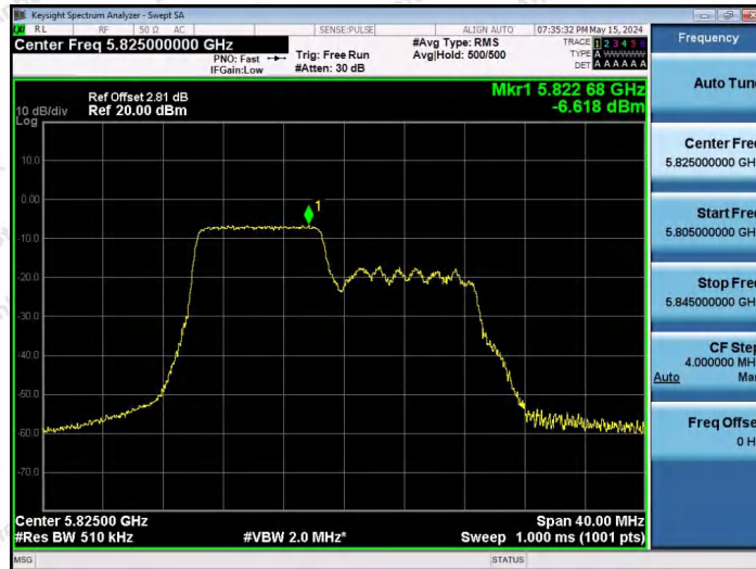
11AX20SISO-Ant1-5825-106Tone-RU53-PASS
