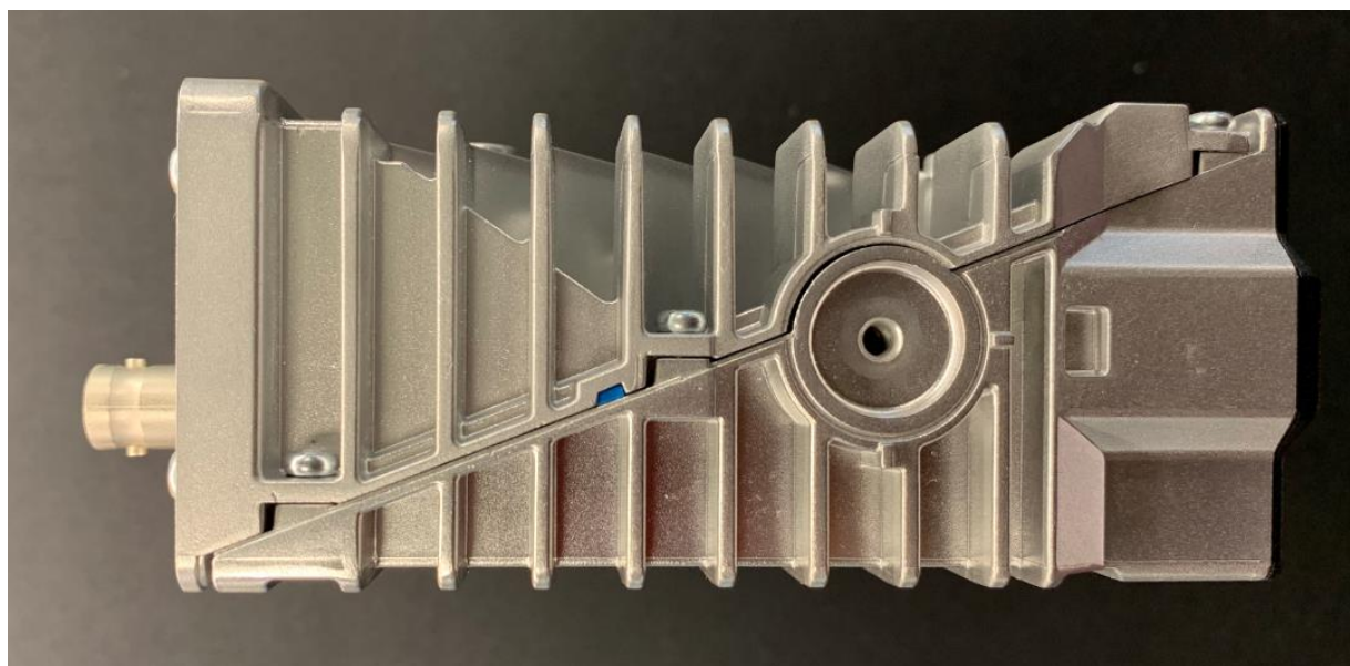
Figure 7. SCG2229 / XX6SCG2229W / 8739A-SCG2229 Top View
