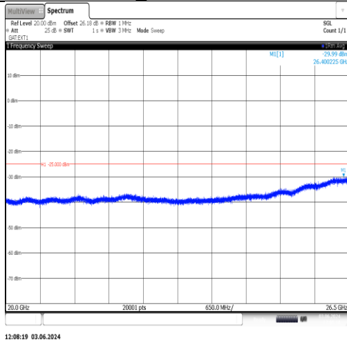
Band41_15MHz_QPSK_41515_1RB#0_20000~26500
