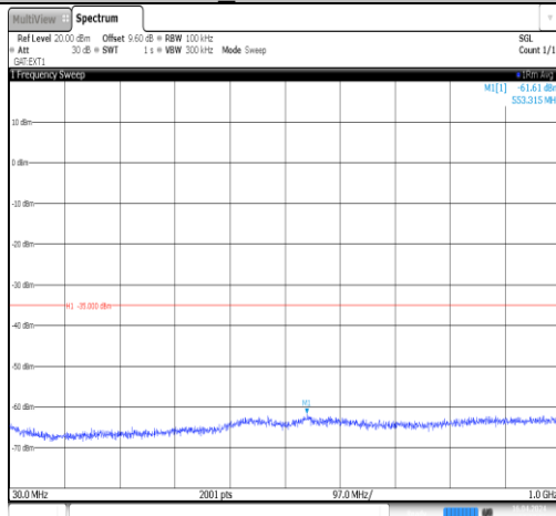
Band41_20MHz_QPSK_39750_1RB#0_30~1000 30~1000
