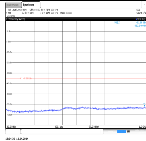
Band41_15MHz_16QAM_39725_1RB#0_30~1000
