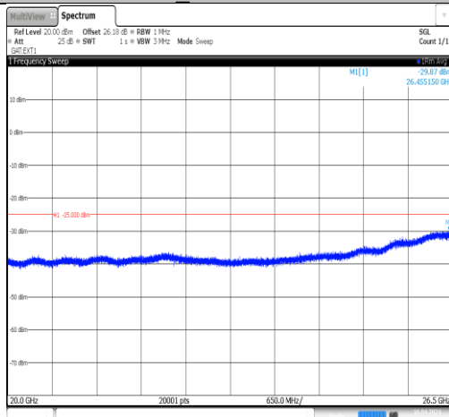
Band41_20MHz_QPSK_39750_1RB#0_20000~26500 6500 20000~26500
