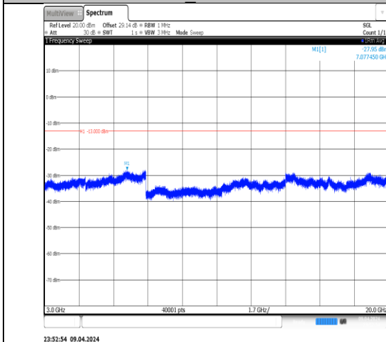
Band66_1.4MHz_QPSK_131979_1RB#0_3000~20000 3000~20000
