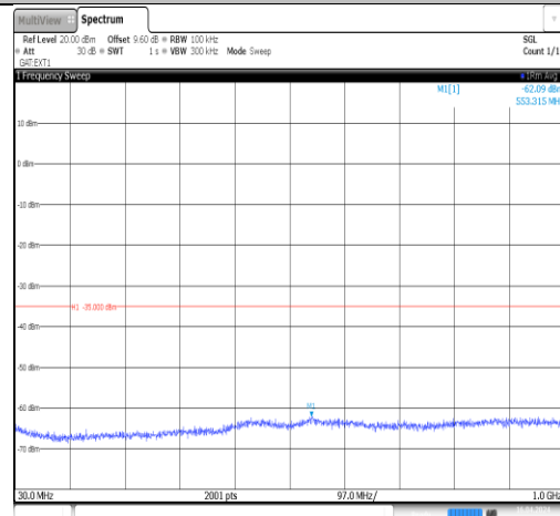
Band41_20MHz_QPSK_40620_1RB#0_30~1000 30~1000
