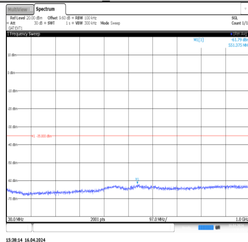
Band41_15MHz_16QAM_41515_1RB#0_30~100 0 30~1000
