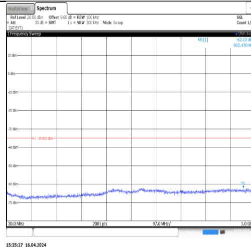
Band41_15MHz_QPSK_40620_1RB#0_30~1000 30~1000
