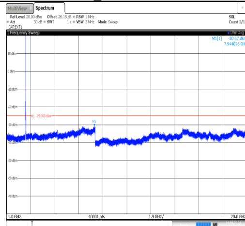
Band41_20MHz_QPSK_39750_1RB#0_1000~20000 1000~20000
