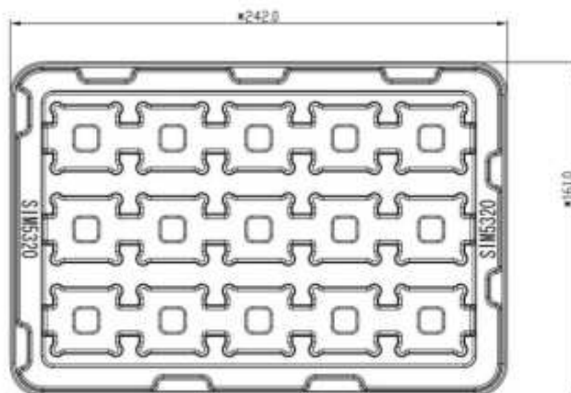
Figure 36: Tray drawing
