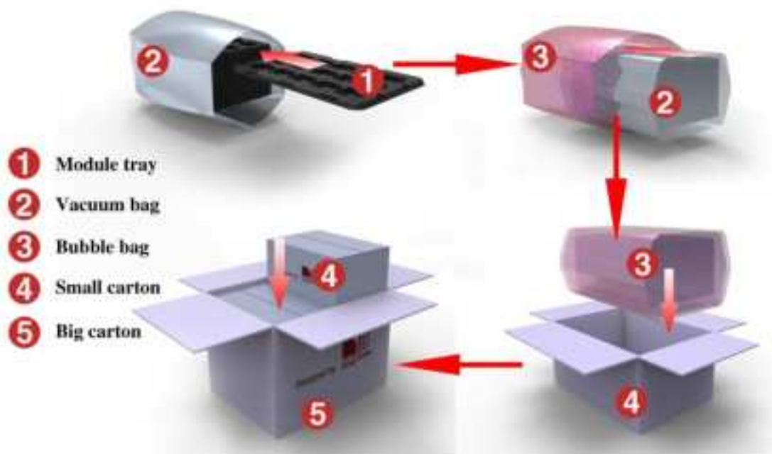
Figure 35: packaging diagram
