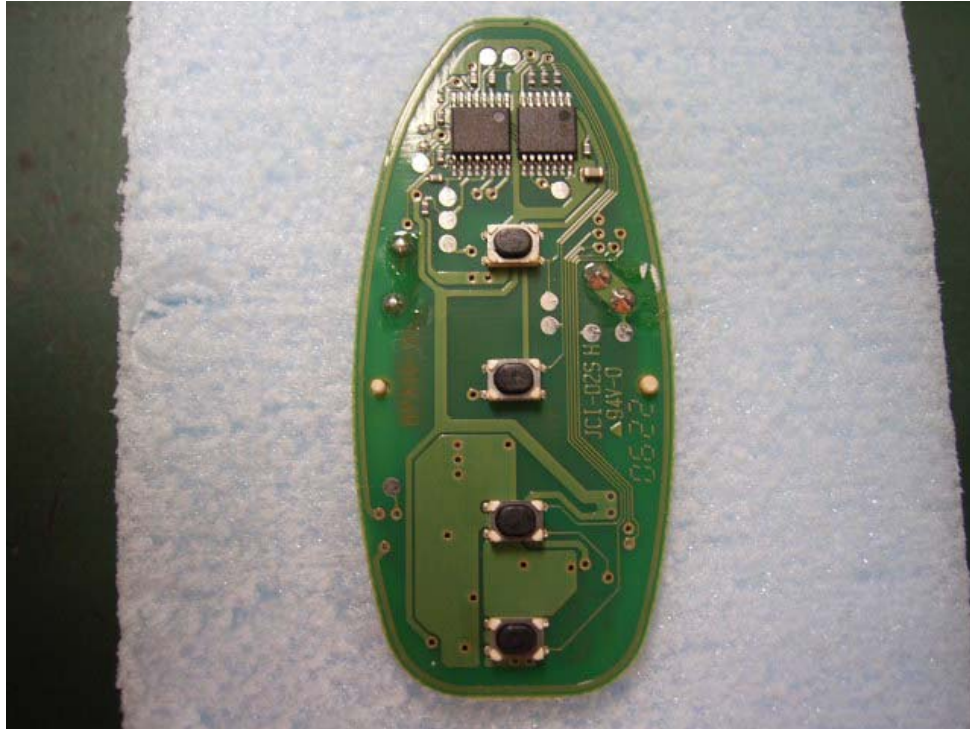
PCB Front
