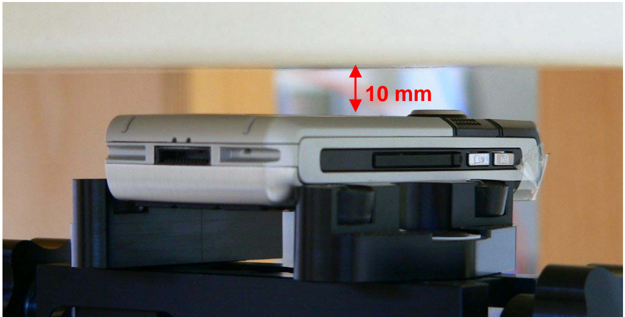
Fig. 31: Body worn configuration Siemens SXG75, GPRS (Class 10) mode without accessory and with activated bluetooth, antenna towards the phantom, gap= 10 mm.
