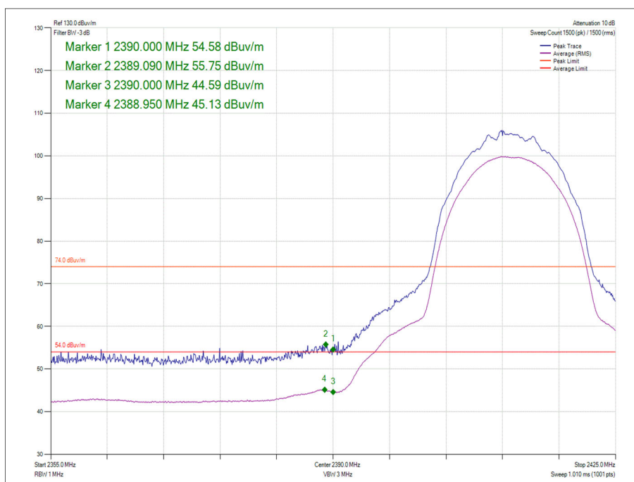
Figure 23 - Data Rate/MCS with the Widest Bandwidth - 5.5 Mbps 2412 MHz - Band Edge Frequency 2390 MHz
