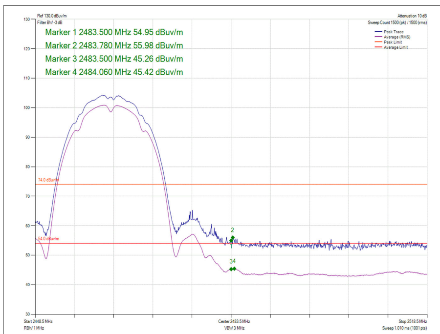
Figure 22 - Data Rate/MCS with the Highest Power - 1 Mbps 2462 MHz - Band Edge Frequency 2483.5 MHz
