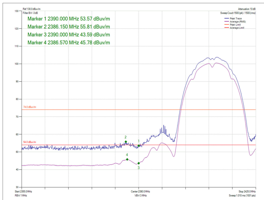
Figure 21 - Data Rate/MCS with the Highest Power - 1 Mbps 2412 MHz - Band Edge Frequency 2390 MHz
