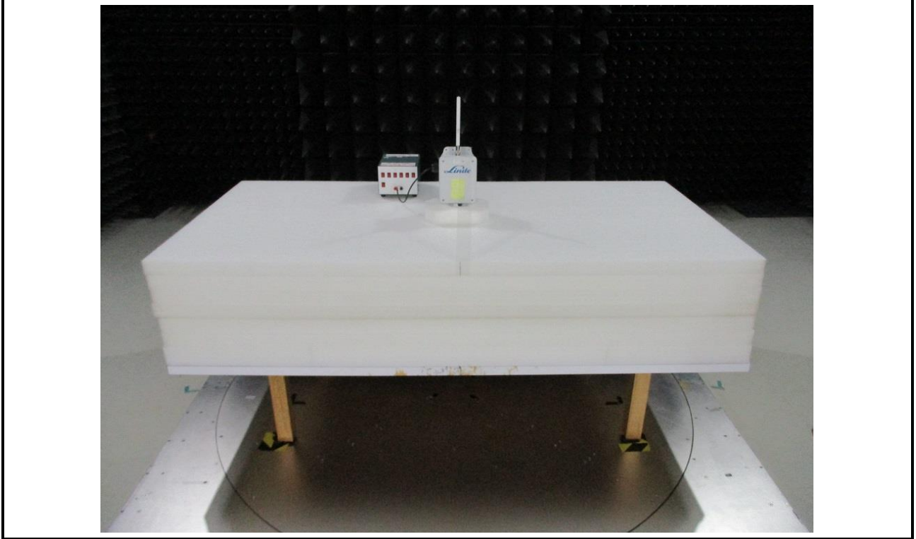
Spurious Emission Below 1GHz Test (For model WSMS-140_C)
