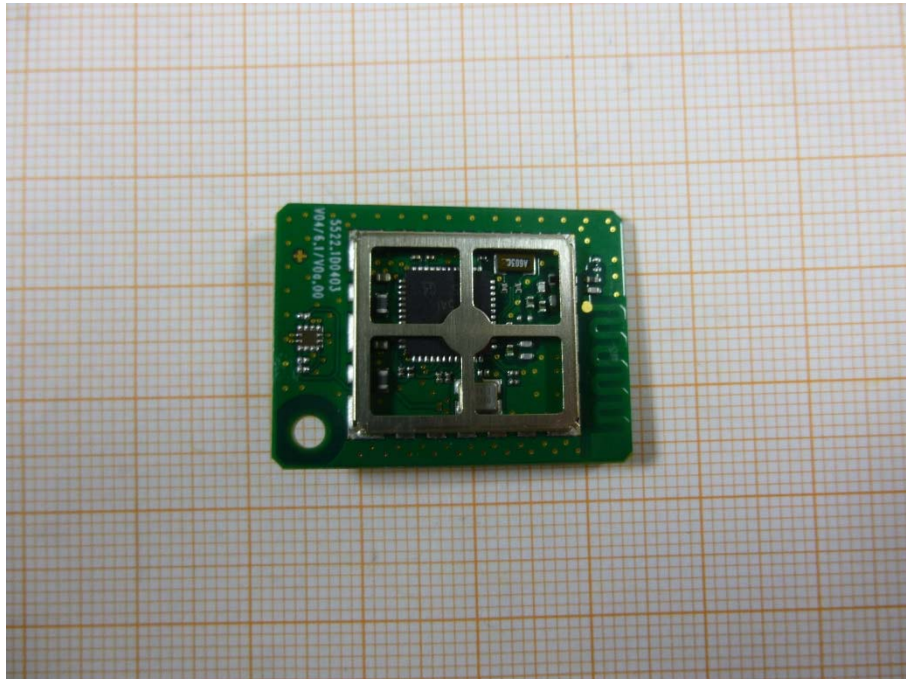
Photo 2: EUT without shielding
