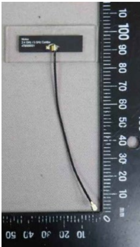
Antenna (Mini-Nanoblade)
