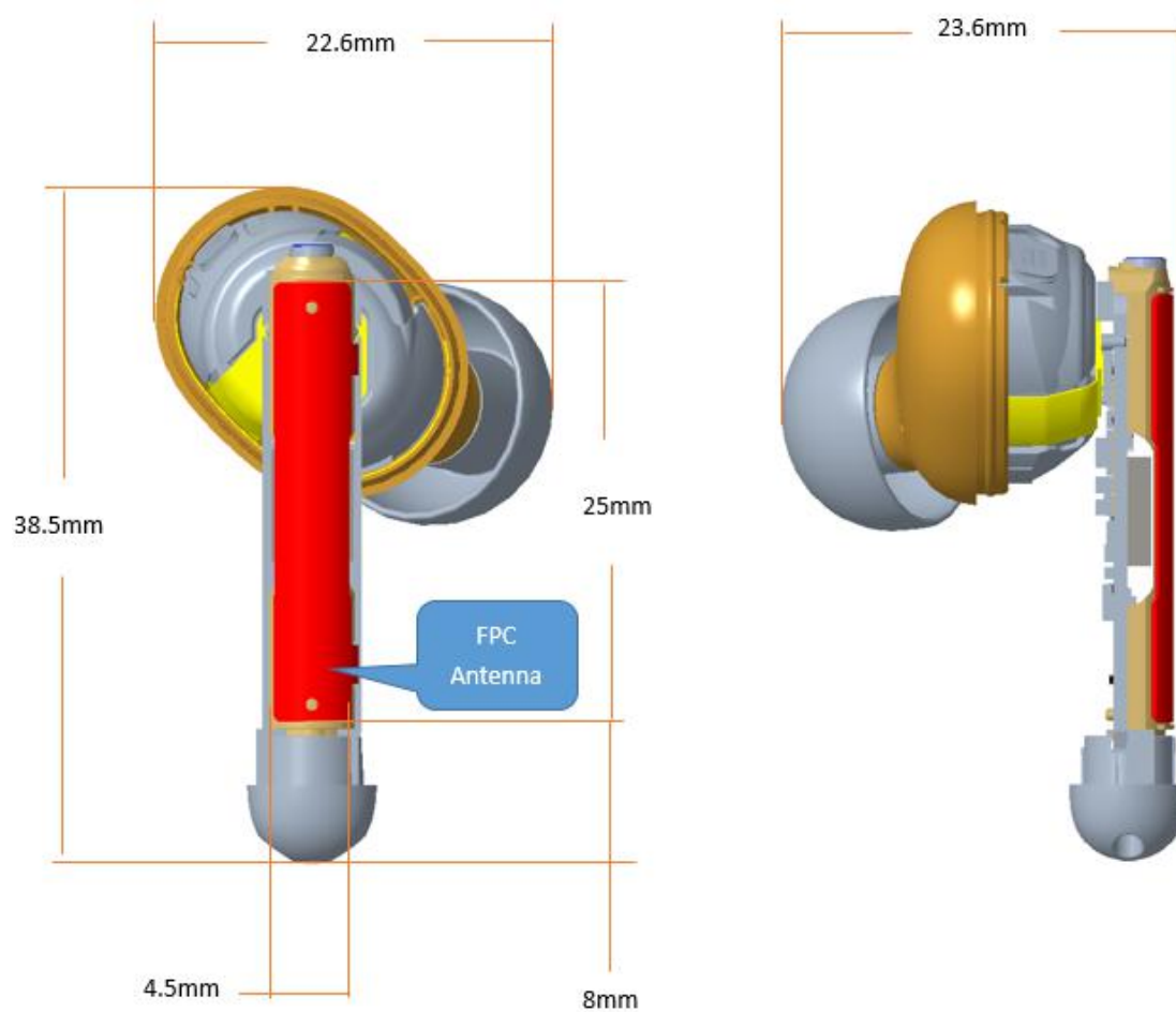
Antenna Location
