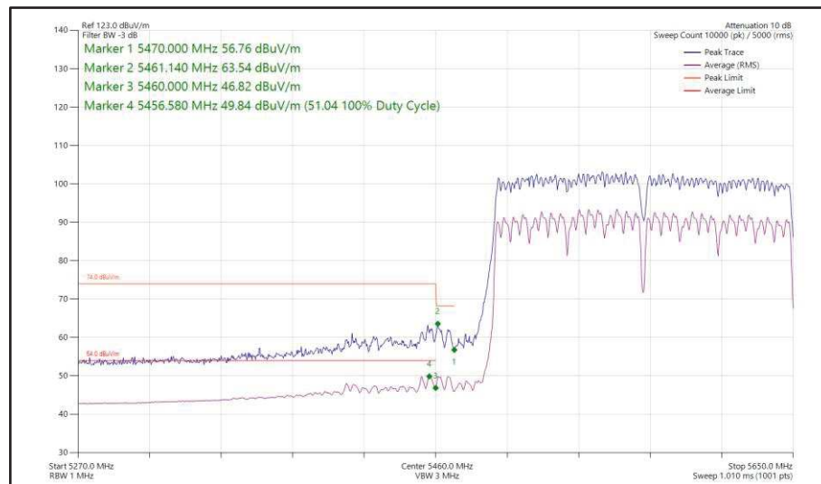
Figure 599 - 802.11ac VHT160, CDD, Core 0 + Core 1 - 5570 MHz Band Edge Frequency 5470 MHz
