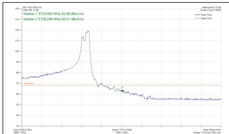
Figure 598 - 802.11ax HE160, RU 106-60, SISO, Core 1 - 5570 MHz Band Edge Frequency 5725 MHz
