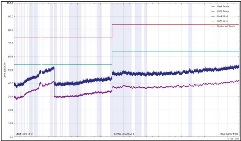
Figure 654 - U-NII-3 - 5745 MHz (CH149), 802.11a, Core 0, 1 GHz to 40 GHz, Horizontal
