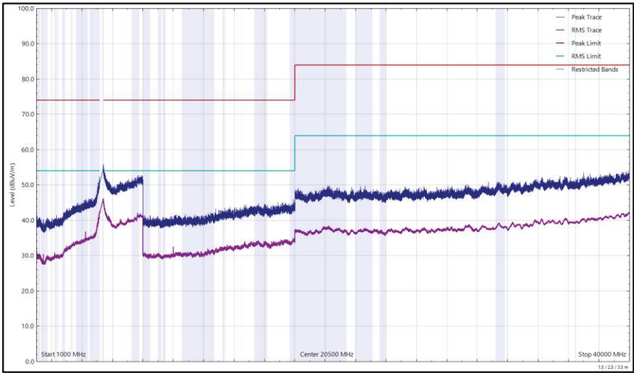
Figure 649 - U-NII-2A - 5320 MHz (CH64), 802.11a, Core 0, 1 GHz to 40 GHz, Vertical
