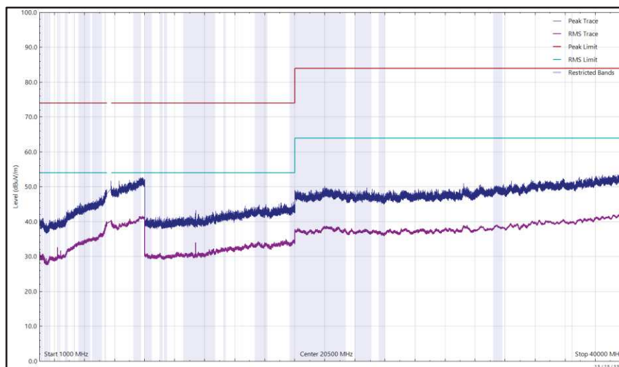
Figure 636 - U-NII-2C - 5700 MHz (CH140), HE20, RU52-37, CDD, Core 0 + Core 1, 1 GHz to 40 GHz, Horizontal
