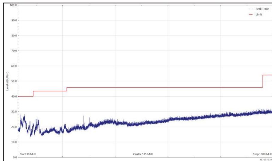
Figure 612 - U-NII-1 - 5180 MHz (CH36), HT20, CDD, Core 0 + Core 1, 30 MHz to 1 GHz, Horizontal (Peak)
