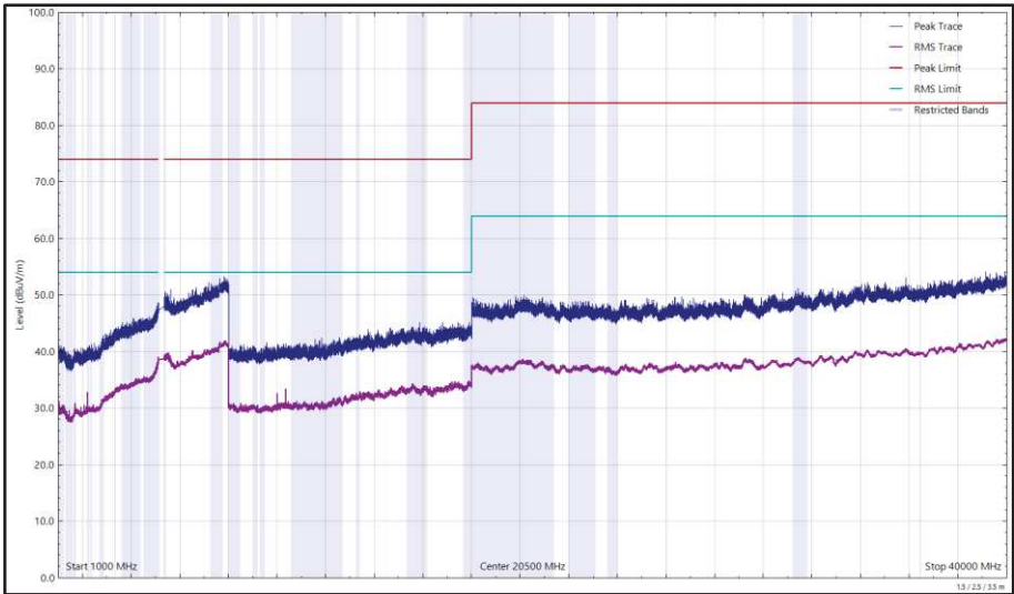
Figure 629 - U-NII-1 - 5180 MHz (CH36), HE20, RU26-0, CDD, Core 0 + Core 1, 1 GHz to 40 GHz, Horizontal
