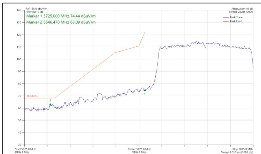
Figure 570 - 802.11ac VHT80, SDM, Core 0 + Core 1 - 5775 MHz Band Edge Frequency 5725 MHz
