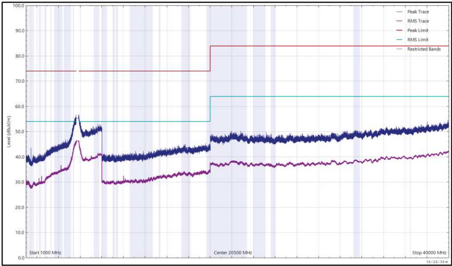
Figure 623 - U-NII-3 - 5745 MHz (CH149), HT20, CDD, Core 0 + Core 1, 1 GHz to 40 GHz, Vertical
