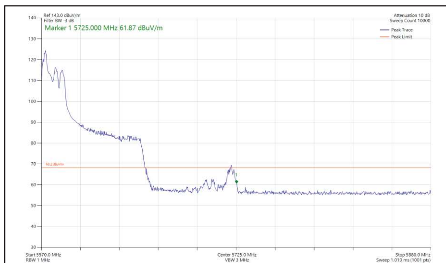
Figure 575 - 802.11ax HE80, RU 52-37, SDM, Core 0 + Core 1 - 5610 MHz Band Edge Frequency 5725 MHz
