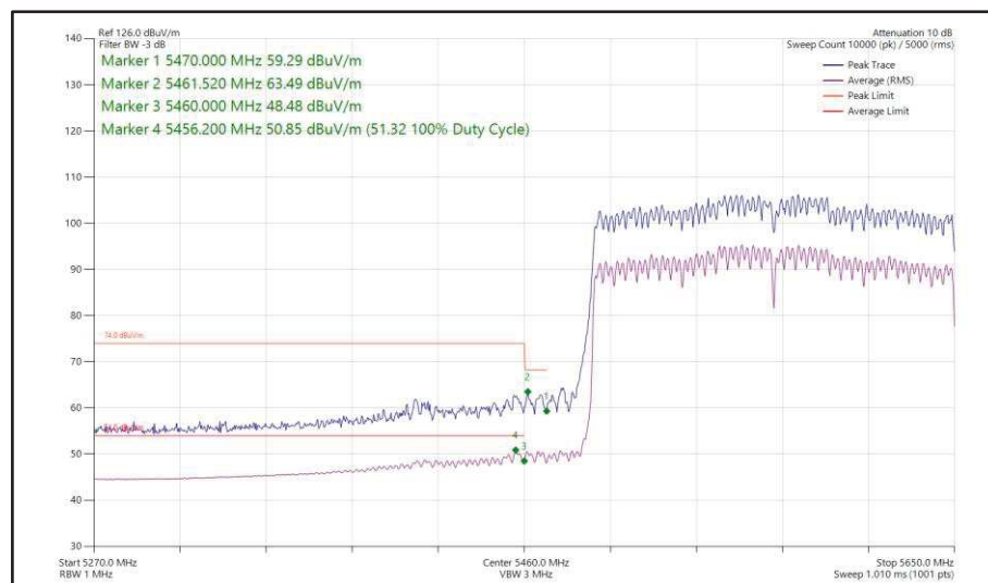
Figure 600 - 802.11ax HE160, SU, CDD, Core 0 + Core 1 - 5570 MHz Band Edge Frequency 5470 MHz
