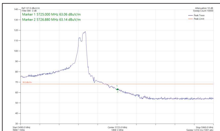
Figure 592 - 802.11ax HE160, RU 106-60, SISO, Core 0 - 5570 MHz Band Edge Frequency 5725 MHz
