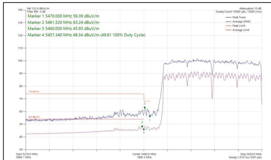
Figure 605 - 802.11ac VHT160, SDM, Core 0 + Core 1 - 5570 MHz Band Edge Frequency 5470 MHz
