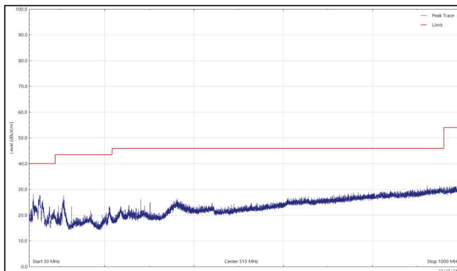
Figure 640 - U-NII-3 - 5825 MHz (CH165), HE20, RU26-0, CDD, Core 0 + Core 1, 30 MHz to 1 GHz, Horizontal (Peak)
