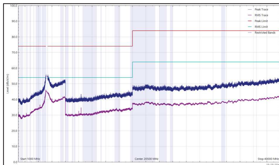
Figure 631 - U-NII-1 - 5180 MHz (CH36), HE20, RU26-0, CDD, Core 0 + Core 1, 1 GHz to 40 GHz, Vertical
