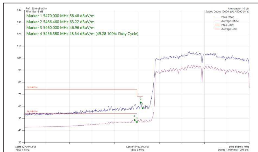
Figure 606 - 802.11ax HE160, SU, SDM, Core 0 + Core 1 - 5570 MHz Band Edge Frequency 5470 MHz
