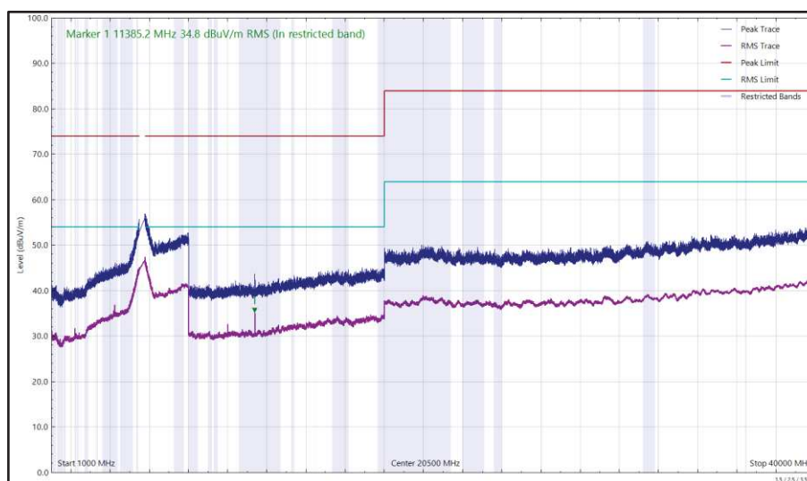
Figure 637 - U-NII-2C - 5700 MHz (CH140), HE20, RU52-37, CDD, Core 0 + Core 1, 1 GHz to 40 GHz, Vertical
