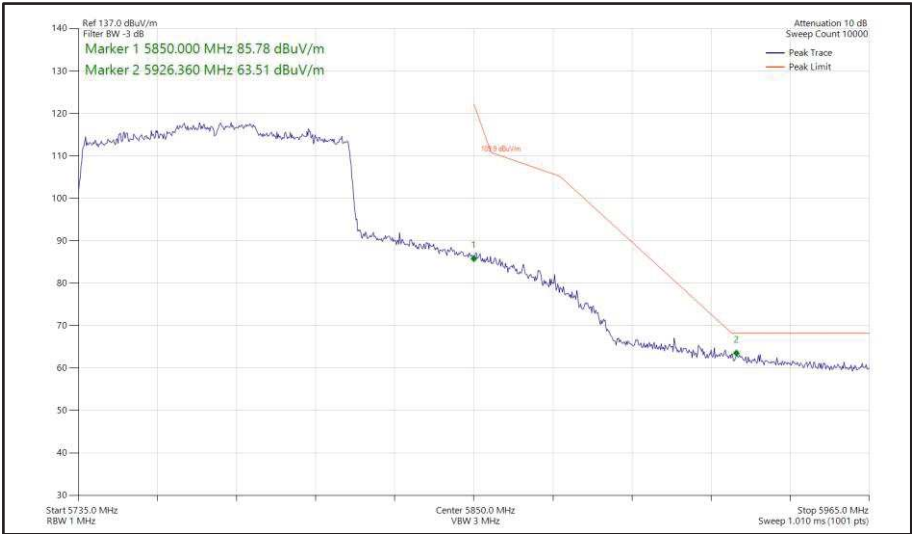
Figure 580 - 802.11ax HE80, SU, SDM, Core 0 + Core 1 - 5775 MHz Band Edge Frequency 5850 MHz
