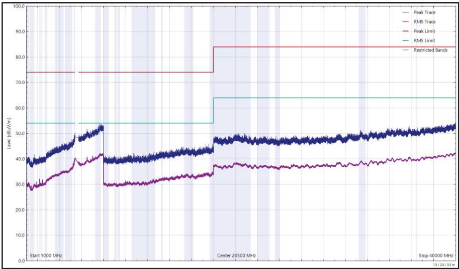
Figure 650 - U-NII-2C - 5500 MHz (CH100), 802.11a, Core 0, 1 GHz to 40 GHz, Horizontal
