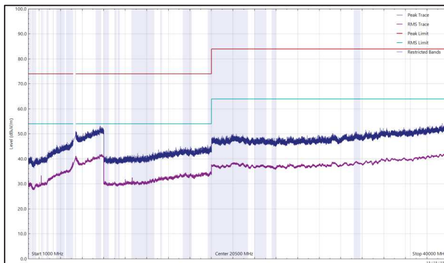
Figure 632 - U-NII-2A - 5320 MHz (CH64), HE20, RU52-37, CDD, Core 0 + Core 1, 1 GHz to 40 GHz, Horizontal
