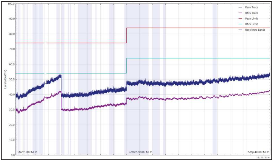
Figure 666 - U-NII-2C - 5500 MHz (CH100), 802.11a, Core 1, 1 GHz to 40 GHz, Horizontal
