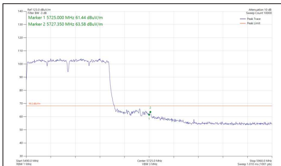
Figure 596 - 802.11ac VHT160, SISO, Core 1 - 5570 MHz Band Edge Frequency 5725 MHz
