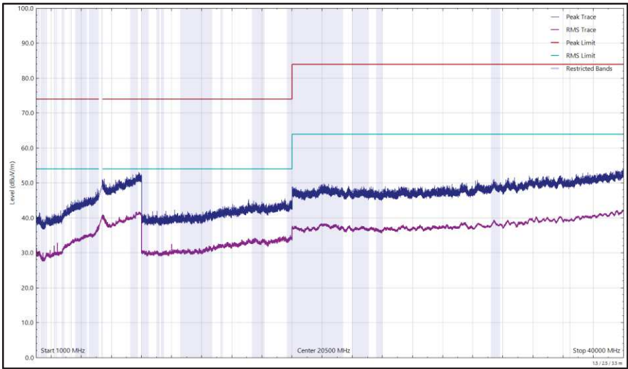
Figure 648 - U-NII-2A - 5320 MHz (CH64), 802.11a, Core 0, 1 GHz to 40 GHz, Horizontal
