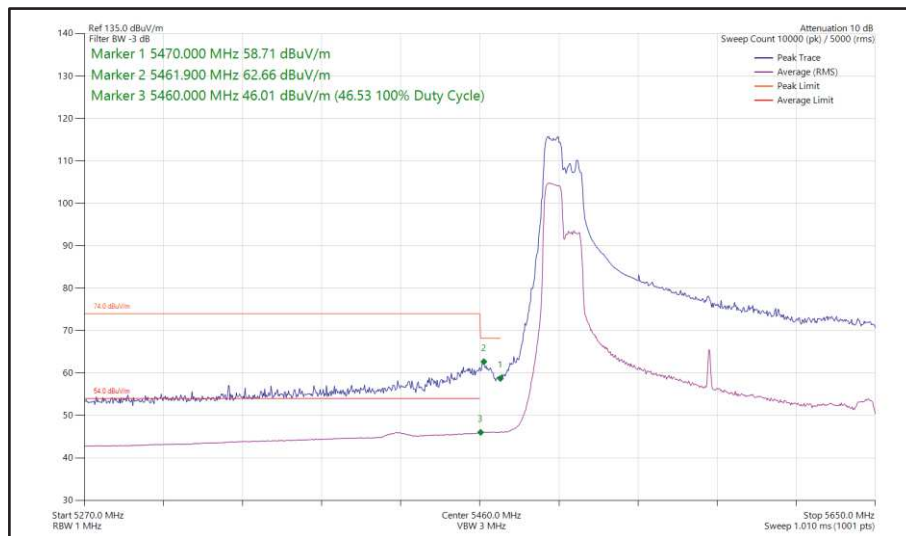
Figure 589 - 802.11ax HE160, RU 106-53, SISO, Core 0 - 5570 MHz Band Edge Frequency 5470 MHz
