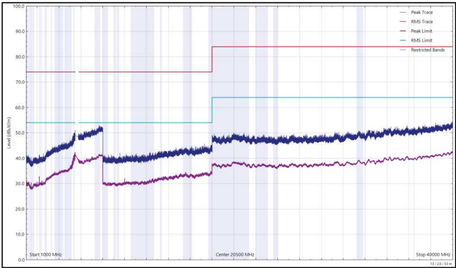
Figure 668 - U-NII-2C - 5700 MHz (CH140), 802.11a, Core 1, 1 GHz to 40 GHz, Horizontal
