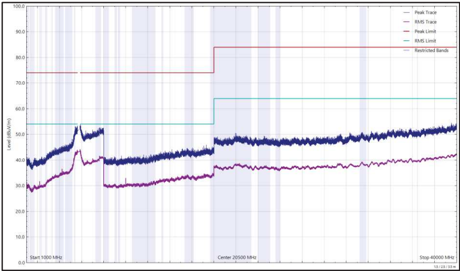
Figure 655 - U-NII-3 - 5745 MHz (CH149), 802.11a, Core 0, 1 GHz to 40 GHz, Vertical
