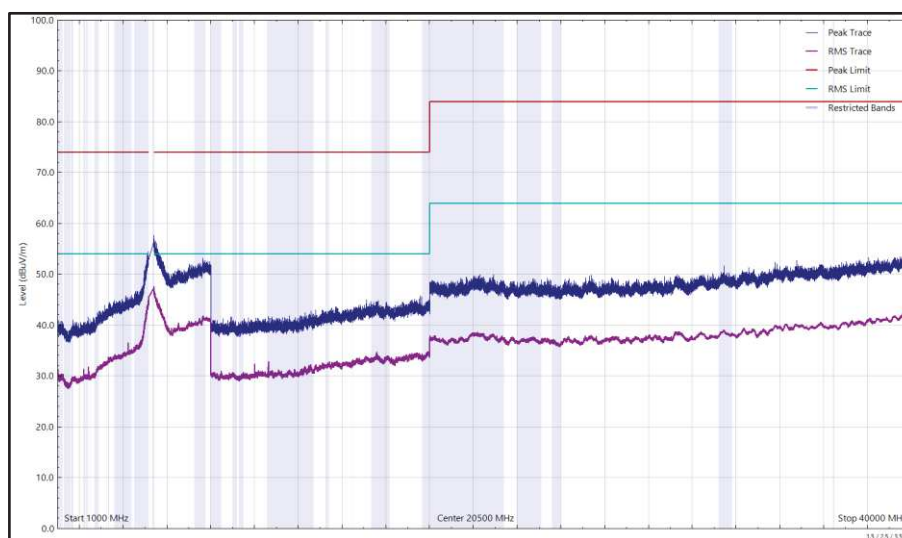
Figure 633 - U-NII-2A - 5320 MHz (CH64), HE20, RU52-37, CDD, Core 0 + Core 1, 1 GHz to 40 GHz, Vertical
