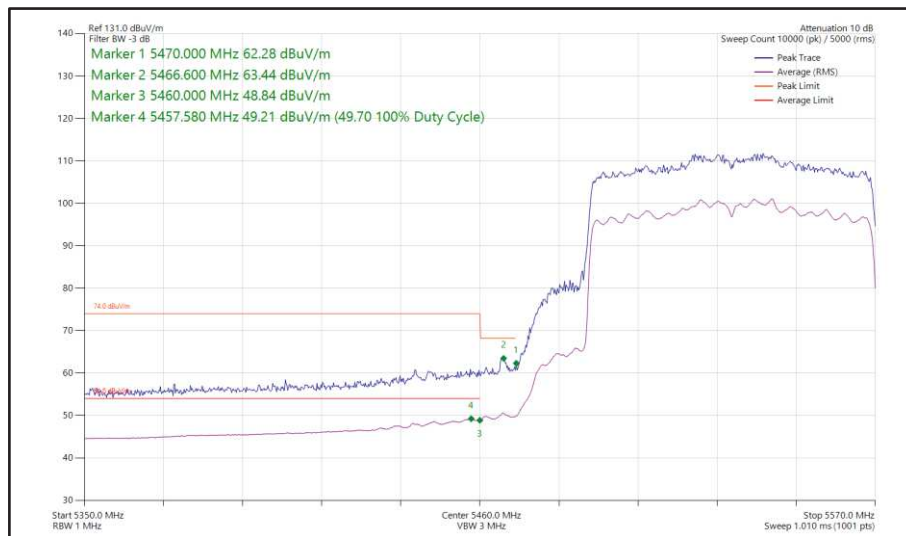
Figure 568 - 802.11ax HE80, SU, SDM, Core 0 + Core 1 - 5530 MHz Band Edge Frequency 5470 MHz
