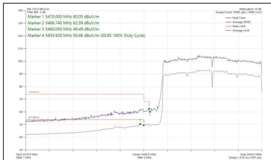
Figure 588 - 802.11ax HE160, SU, SISO, Core 0 - 5570 MHz Band Edge Frequency 5470 MHz
