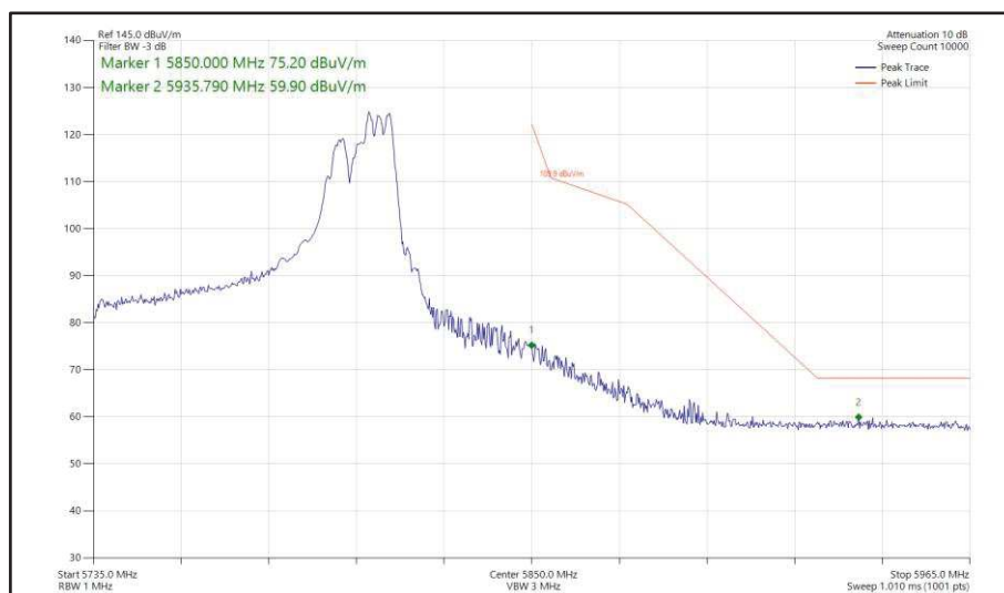
Figure 566 - 802.11ax HE80, RU 106-60, CDD, Core 0 + Core 1 - 5775 MHz Band Edge Frequency 5850 MHz
