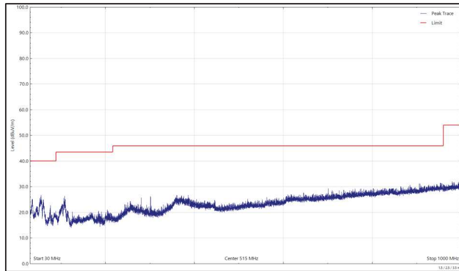
Figure 672 - U-NII-3 - 5825 MHz (CH165), 802.11a, Core 1, 30 MHz to 1 GHz, Horizontal (Peak)
