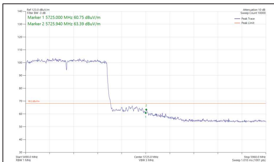
Figure 591 - 802.11ax HE160, SU, SISO, Core 0 - 5570 MHz Band Edge Frequency 5725 MHz
