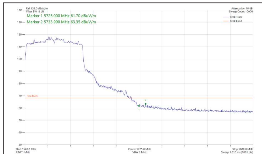
Figure 573 - 802.11ac VHT80, SDM, Core 0 + Core 1 - 5610 MHz Band Edge Frequency 5725 MHz
