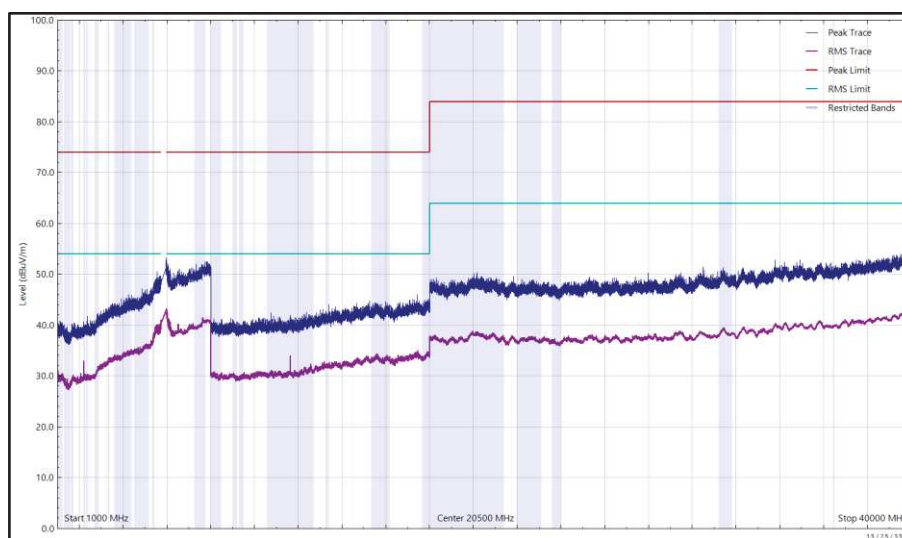
Figure 641 - U-NII-3 - 5825 MHz (CH165), HE20, RU26-0, CDD, Core 0 + Core 1, 1 GHz to 40 GHz, Horizontal
