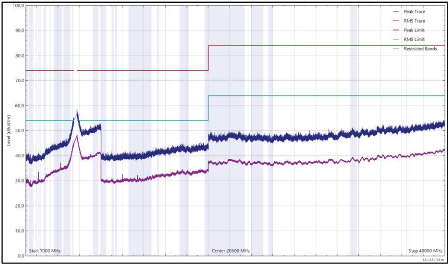
Figure 621 - U-NII-2C - 5700 MHz (CH140), HT20, CDD, Core 0 + Core 1, 1 GHz to 40 GHz, Vertical
