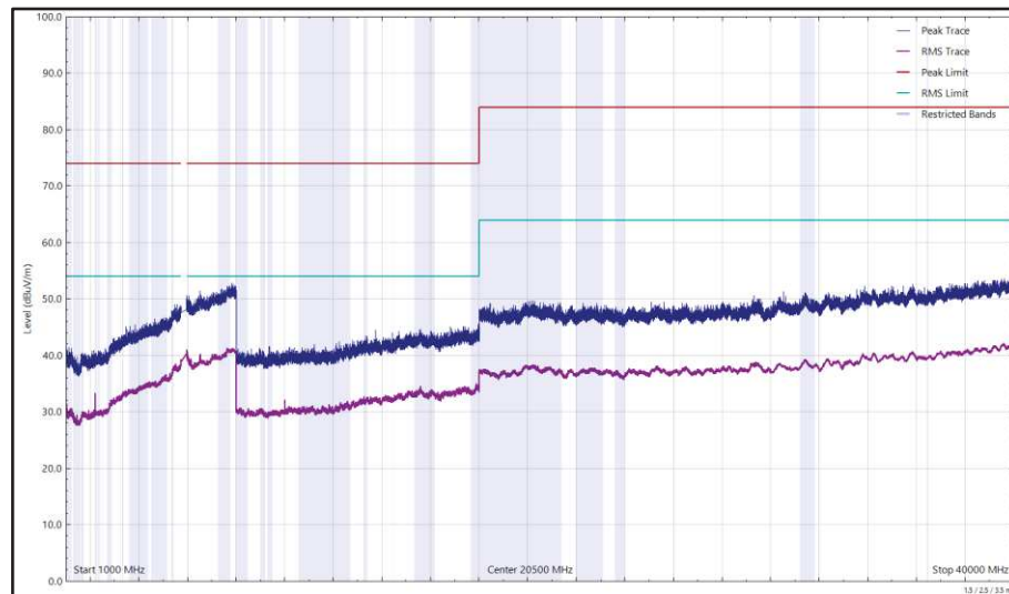
Figure 673 - U-NII-3 - 5825 MHz (CH165), 802.11a, Core 1, 1 GHz to 40 GHz, Horizontal
