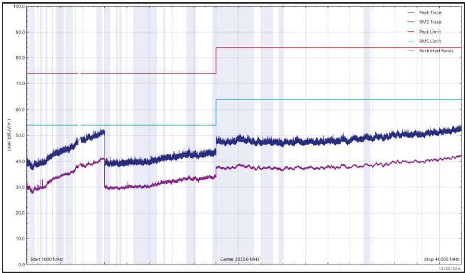
Figure 670 - U-NII-3 - 5745 MHz (CH149), 802.11a, Core 1, 1 GHz to 40 GHz, Horizontal
