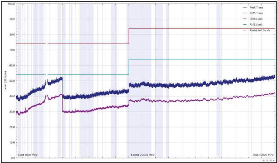
Figure 652 - U-NII-2C - 5700 MHz (CH140), 802.11a, Core 0, 1 GHz to 40 GHz, Horizontal
