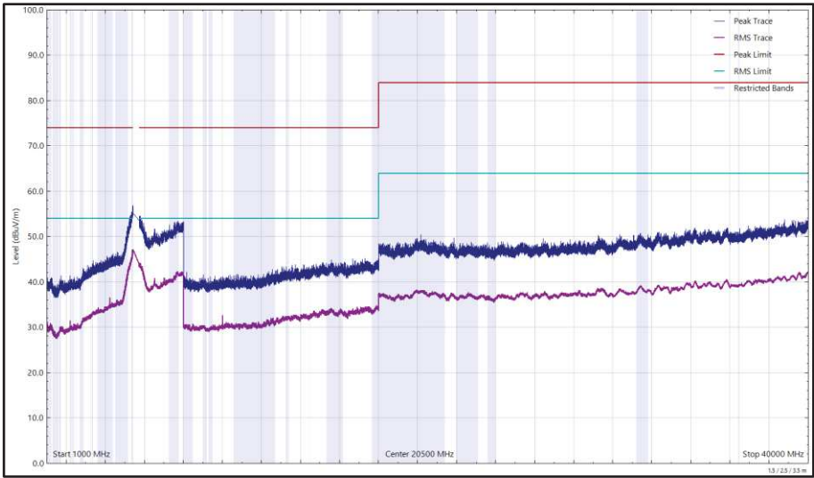
Figure 619 - U-NII-2C - 5500 MHz (CH100), HT20, CDD, Core 0 + Core 1, 1 GHz to 40 GHz, Vertical
