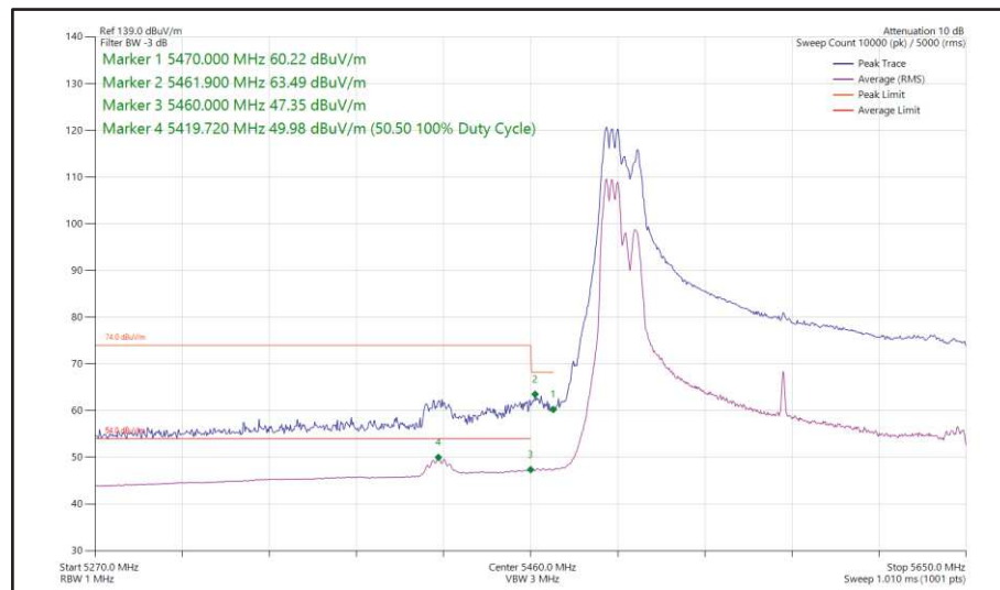
Figure 601 - 802.11ax HE160, RU 106-53, CDD, Core 0 + Core 1 - 5570 MHz Band Edge Frequency 5470 MHz
