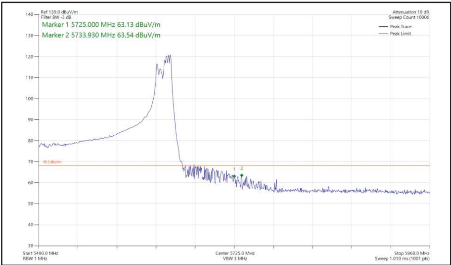
Figure 610 - 802.11ax HE160, RU 106-60, SDM, Core 0 + Core 1 - 5570 MHz Band Edge Frequency 5725 MHz
