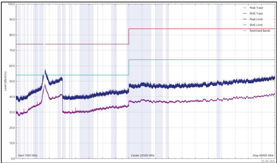
Figure 617 - U-NII-2A - 5320 MHz (CH64), HT20, CDD, Core 0 + Core 1, 1 GHz to 40 GHz, Vertical
