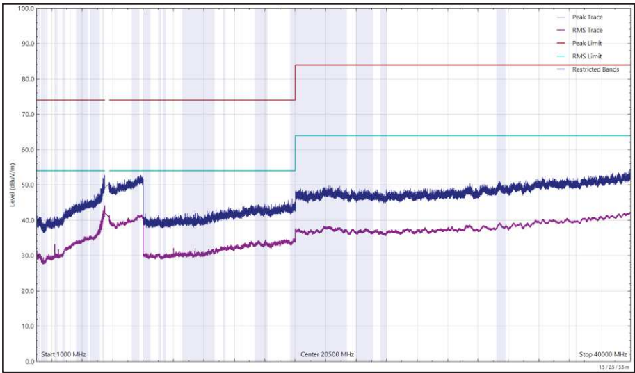
Figure 620 - U-NII-2C - 5700 MHz (CH140), HT20, CDD, Core 0 + Core 1, 1 GHz to 40 GHz, Horizontal
