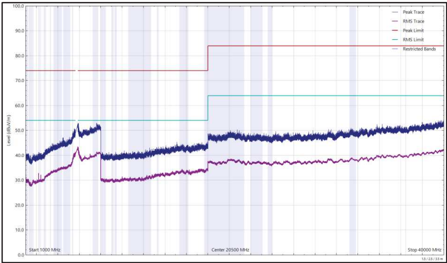
Figure 622 - U-NII-3 - 5745 MHz (CH149), HT20, CDD, Core 0 + Core 1, 1 GHz to 40 GHz, Horizontal
