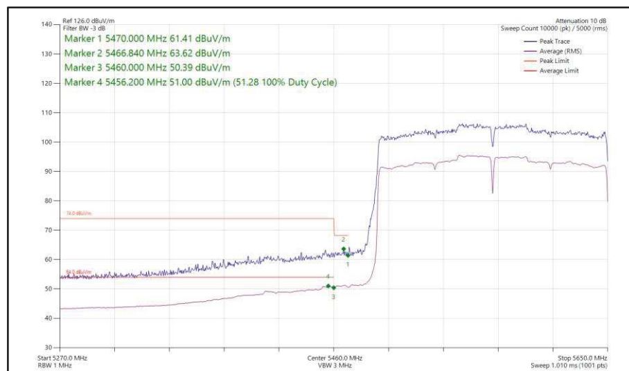
Figure 594 - 802.11ax HE160, SU, SISO, Core 1 - 5570 MHz Band Edge Frequency 5470 MHz
