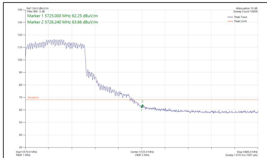
Figure 559 - 802.11ax HE80, SU, CDD, Core 0 + Core 1 - 5610 MHz Band Edge Frequency 5725 MHz
