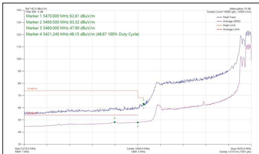
Figure 607 - 802.11ax HE160, RU 106-60, SDM, Core 0 + Core 1 - 5570 MHz Band Edge Frequency 5470 MHz
