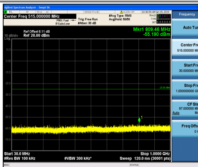
Band7_5MHz_16QAM_21100_1RB#0
