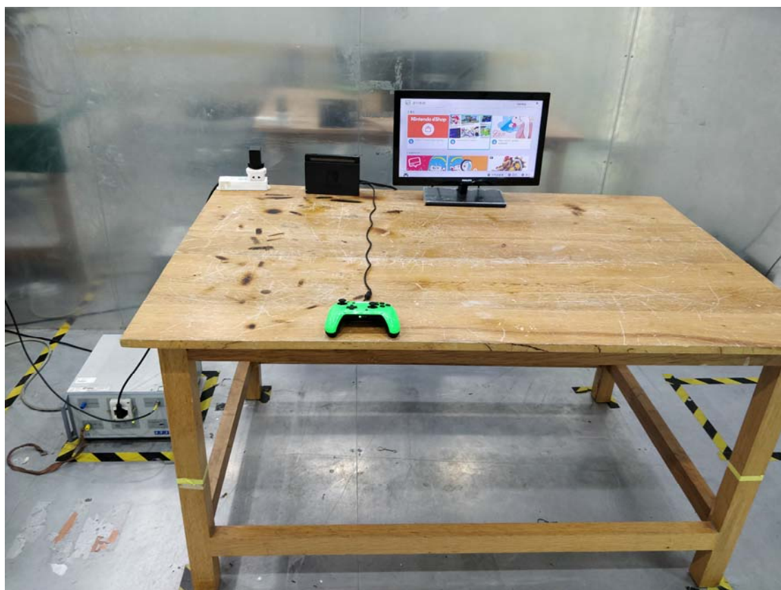
Conduction Setup photo
