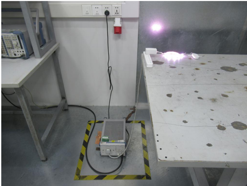
FCC ID: 2AQA6-H6188 Photo of Power Line Conducted Emission Test
