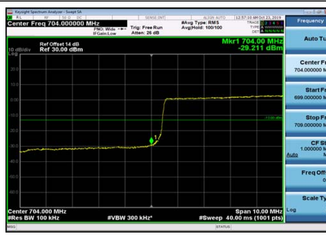
LowRange_FDD17_10MHz_709_fullRB _Low_QPSK
