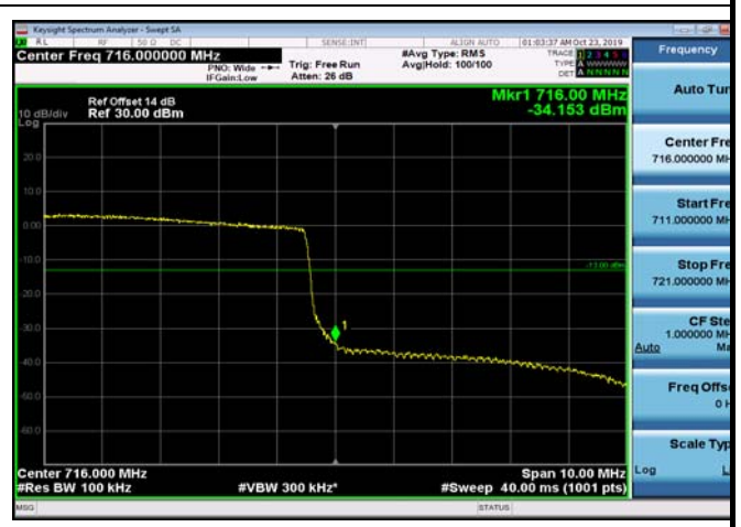
HighRange_FDD17_10MHz_711_fullRB _High_Q16
