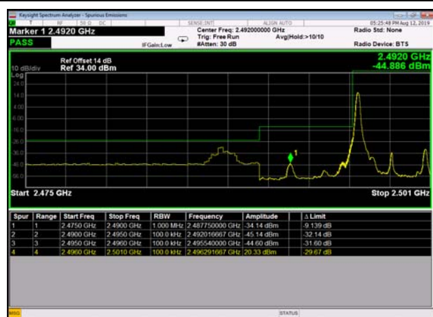
LowRange_TDD41_5MHz_2498.5_fullRB _LowQPSK
