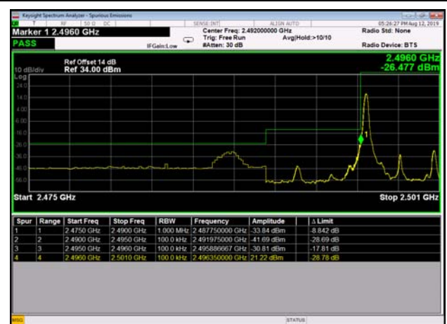
LowRange_TDD41_5MHz_2498.5_fullRB _LowQ16
