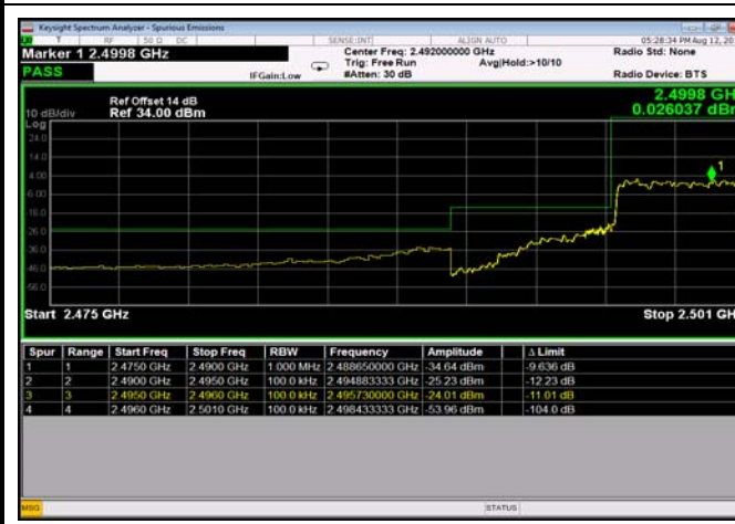
LowRange_TDD41_5MHz_2498.5_fullRB _LowQPSK
