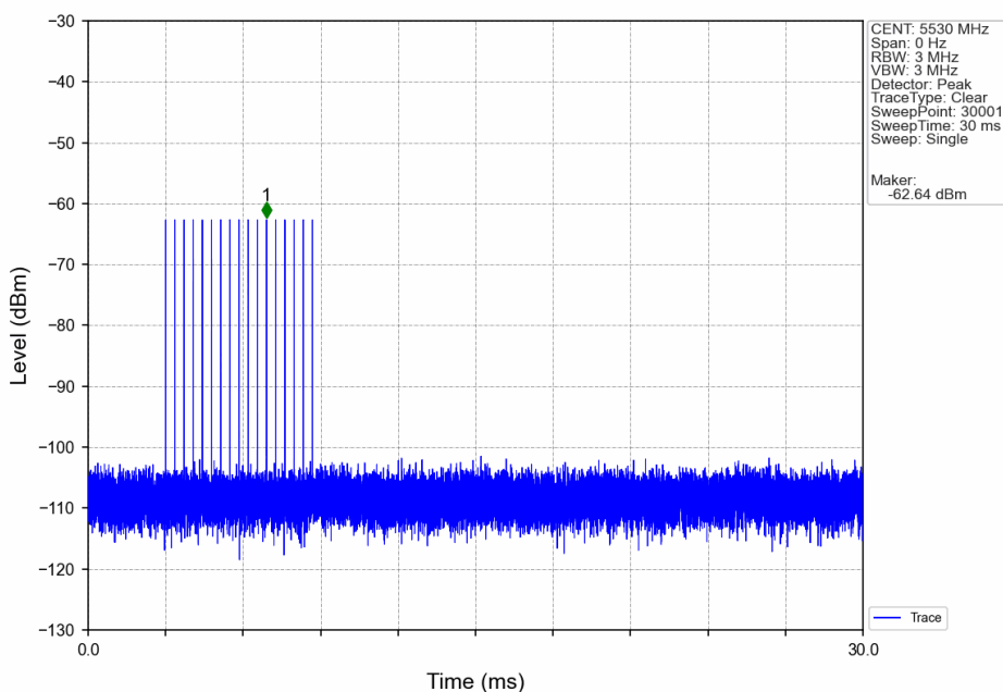
Signal Calibration 802.11ax(HE80) 2C 5530MHz RadarType3 Trial0
