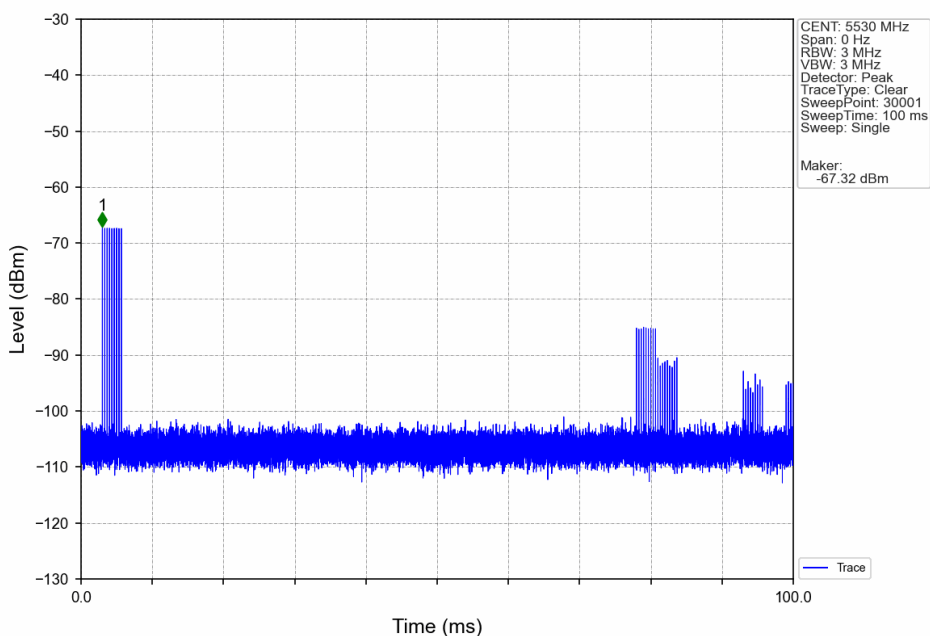
Signal Calibration 802.11ax(HE80) 2C 5530MHz RadarType6 Trial0
