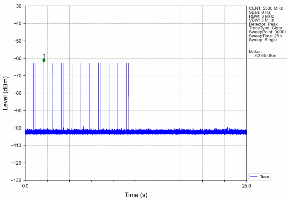
Signal Calibration 802.11ax(HE80) 2C 5530MHz RadarType5 Trial0
