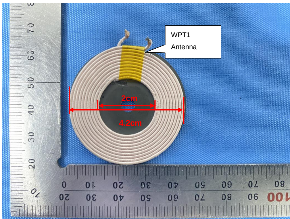
WPT1 Antenna
