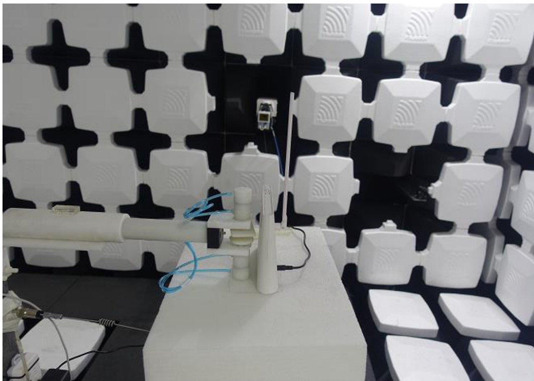
Radiated Spurious Emission (18GHz to26.5GHz)
