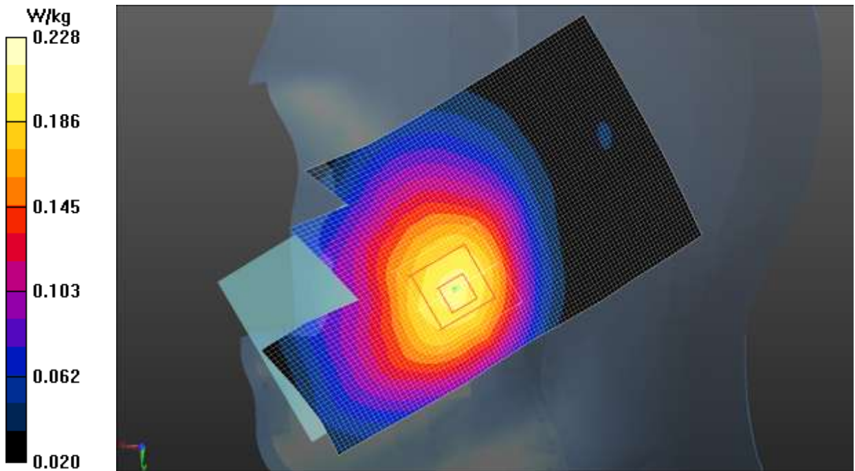
Fig.31 LTE Band 26
