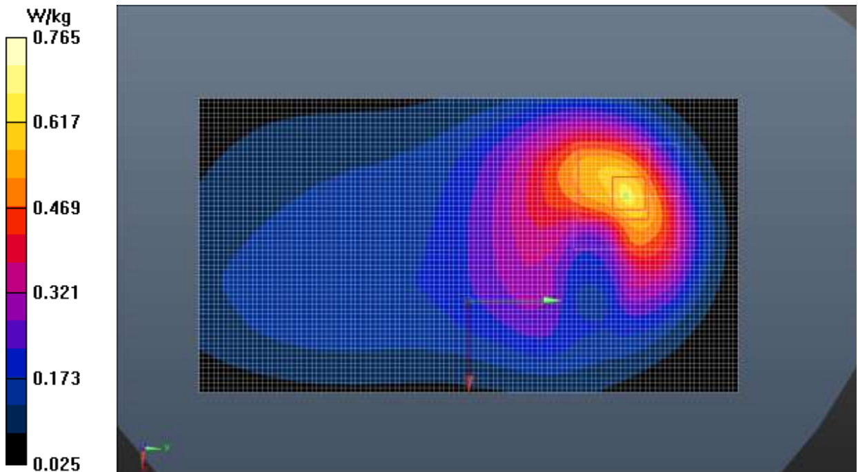
Fig.22 LTE Band 5
