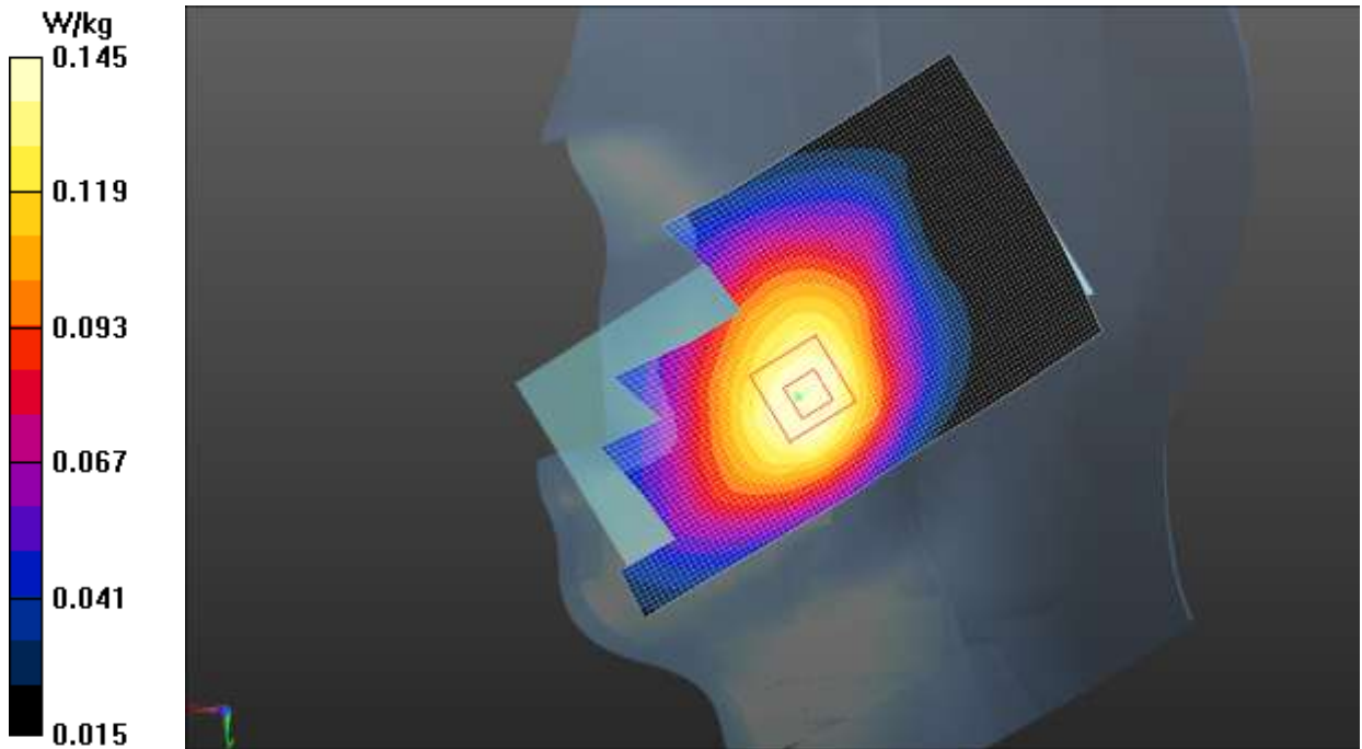
Fig.27 LTE Band 13
