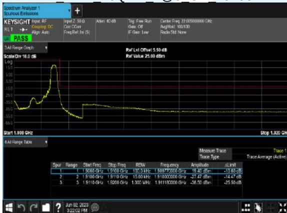
B2 1.4M 16QAM 1@5 CH 19193
