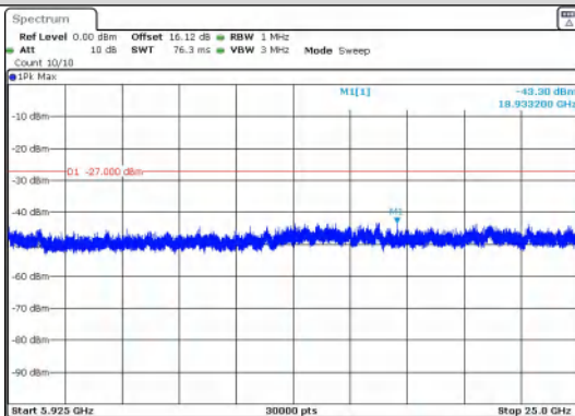
Out Of Band Emission IEEE 802.11a_Channel 157_20MHz_Antenna 0
