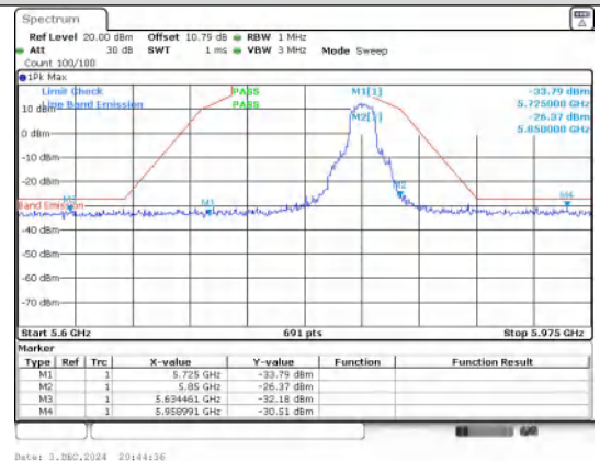
Out Of Band Emission IEEE 802.11a_Channel 165_20MHz_Antenna 1
