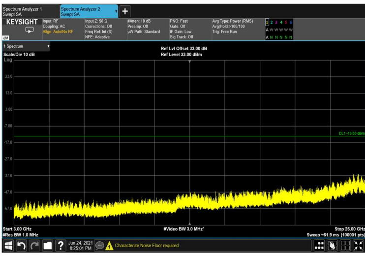
Figure 413: 3GHz-26GHz
