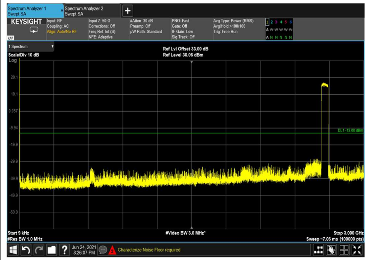
Figure 418: 9kHz-3GHz
