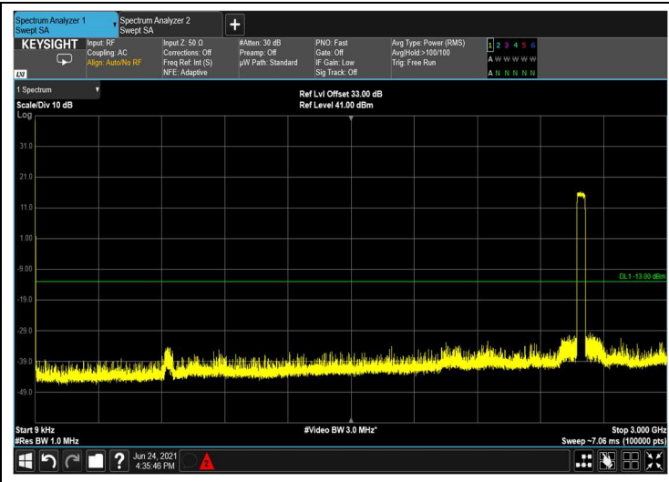
Figure 422: 9kHz-3GHz
