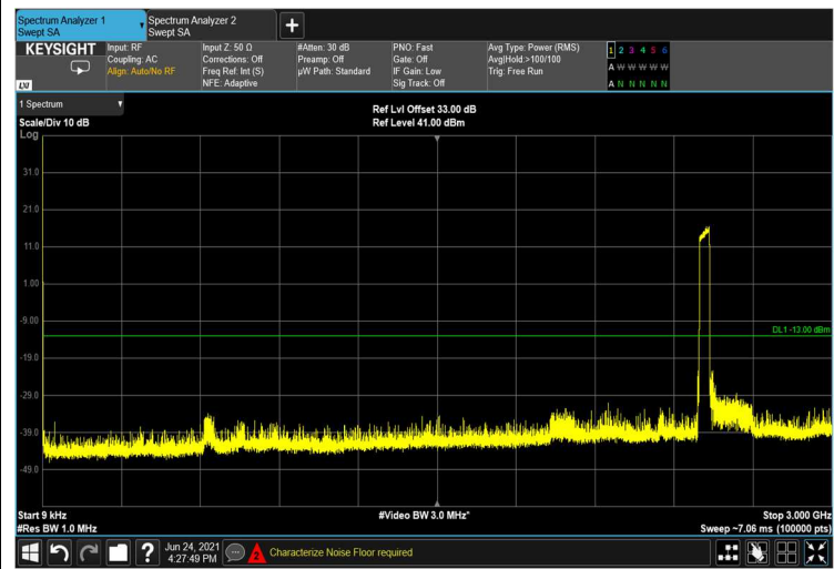
Figure 432: 9kHz-3GHz
