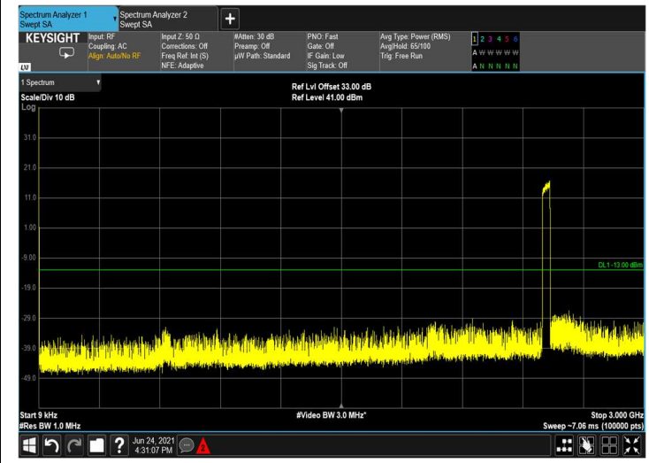
Figure 402: 9kHz-3GHz
