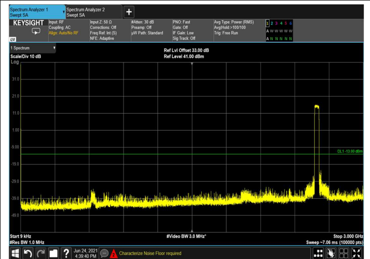
Figure 398: 9kHz-3GHz
