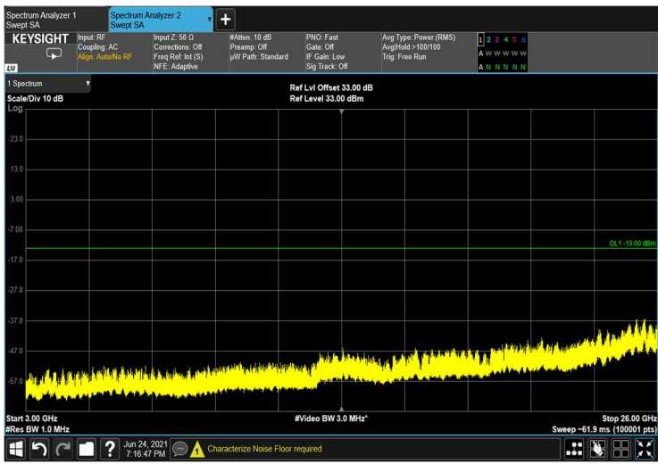
Figure 411: 3GHz-26GHz
