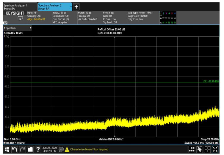
Figure 391: 3GHz-26GHz
