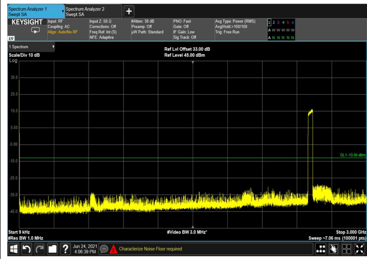
Figure 390: 9kHz-3GHz
