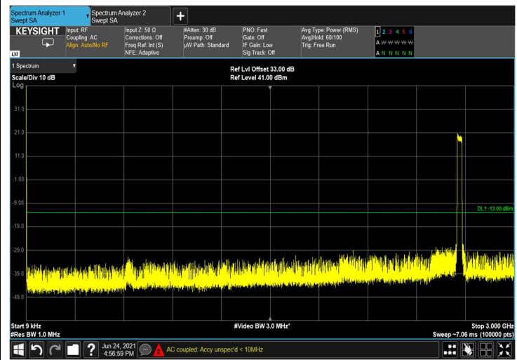
Spurious Emissions at Antenna Terminal QPSK 40MHz B.W.; 2670.0MHz, 15kHz
