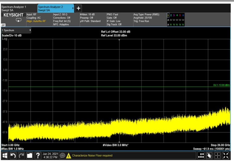
Figure 423: 3GHz-26GHz
