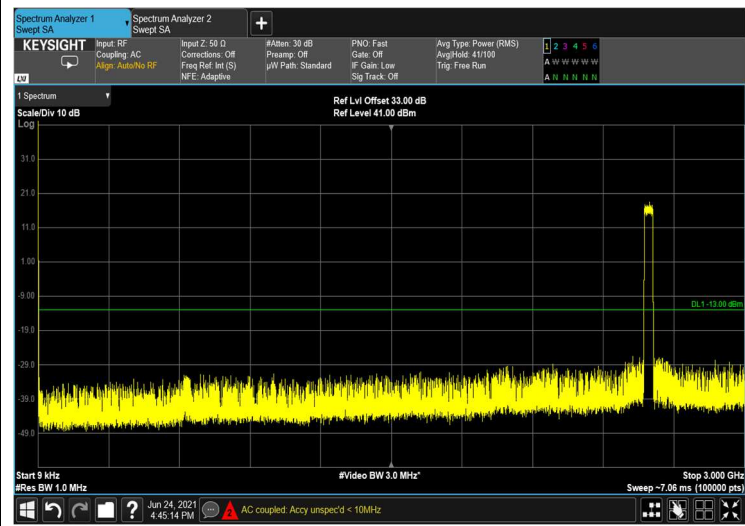
Spurious Emissions at Antenna Terminal 256QAM 40MHz B.W.; 2593.0MHz, 60kHz
