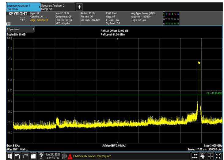
Spurious Emissions at Antenna Terminal QPSK 40MHz B.W.; 2670.0MHz, 30kHz
