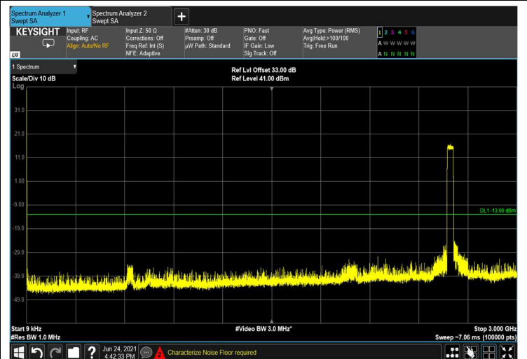
Figure 434: 9kHz-3GHz
