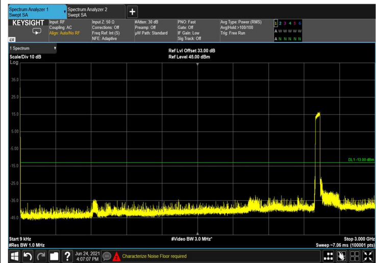
Figure 396: 9kHz-3GHz
