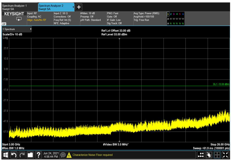
Spurious Emissions at Antenna Terminal QPSK 40MHz B.W.; 2670.0MHz, 15kHz
