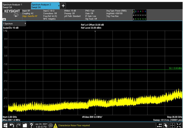
Figure 393: 3GHz-26GHz
