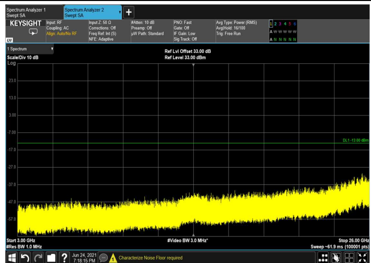
Figure 417: 3GHz-26GHz
