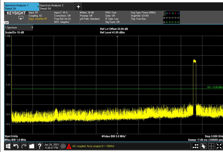
Figure 392: 9kHz-3GHz
