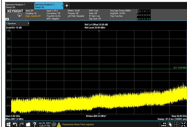
Figure 433: 3GHz-26GHz
