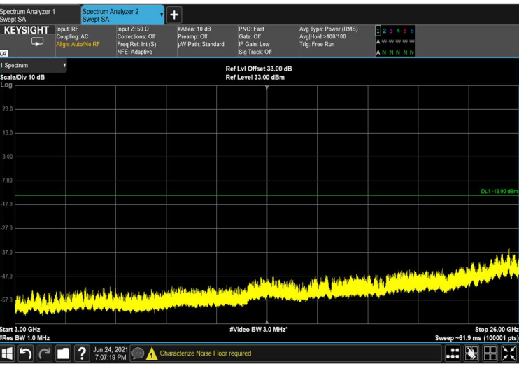
Figure 415: 3GHz-26GHz
