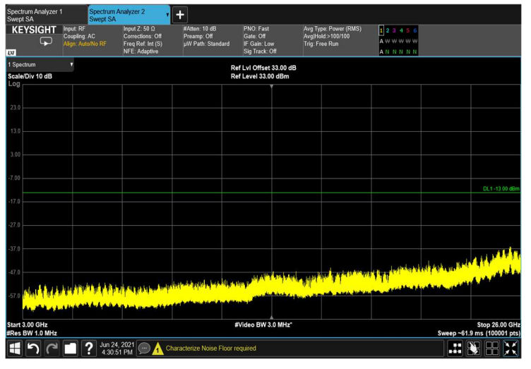
Figure 403: 3GHz-26GHz
