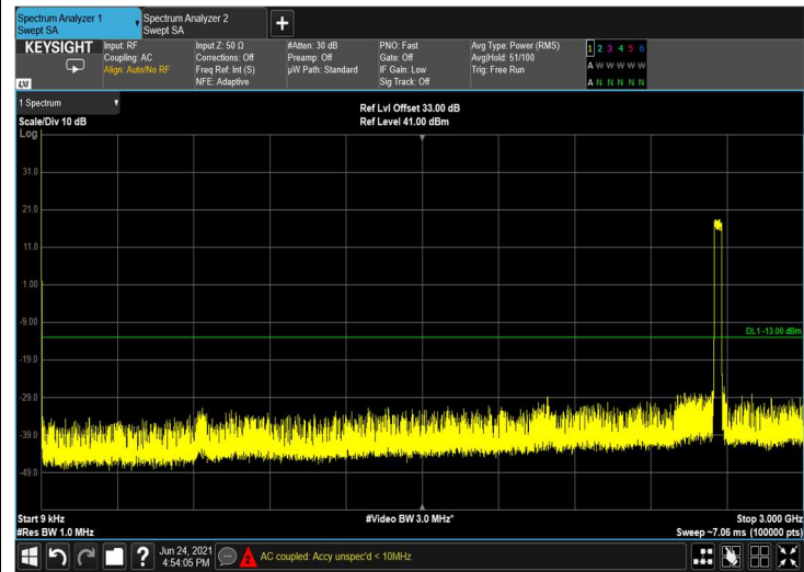
Figure 400: 9kHz-3GHz
