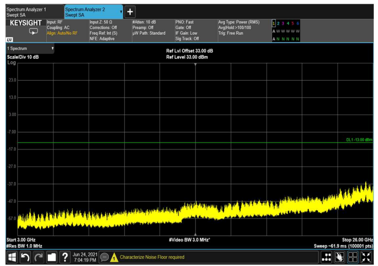
Figure 409: 3GHz-26GHz
