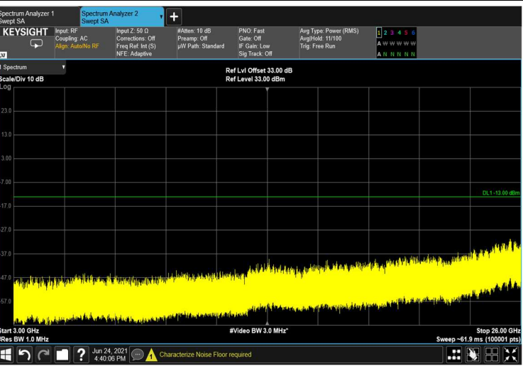
Figure 399: 3GHz-26GHz
