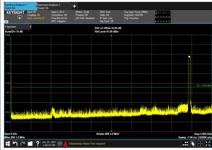
Spurious Emissions at Antenna Terminal 256QAM 40MHz B.W.; 2670.0MHz, 60kHz
