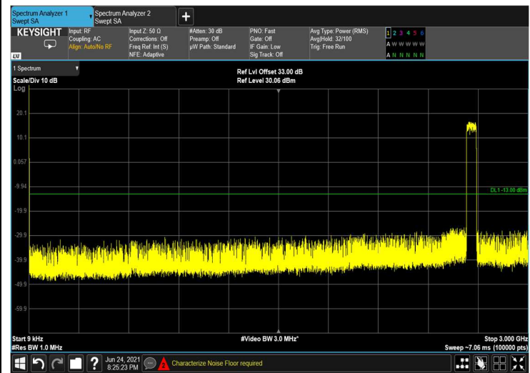
Figure 412: 9kHz-3GHz
