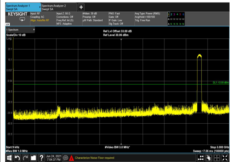
Figure 408: 9kHz-3GHz
