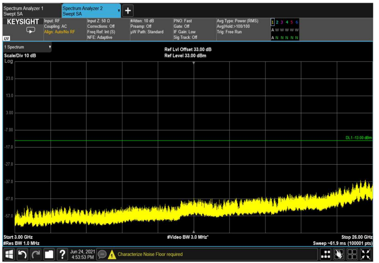
Figure 401: 3GHz-26GHz
