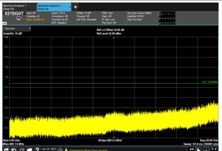
Figure 435: 3GHz-26GHz
