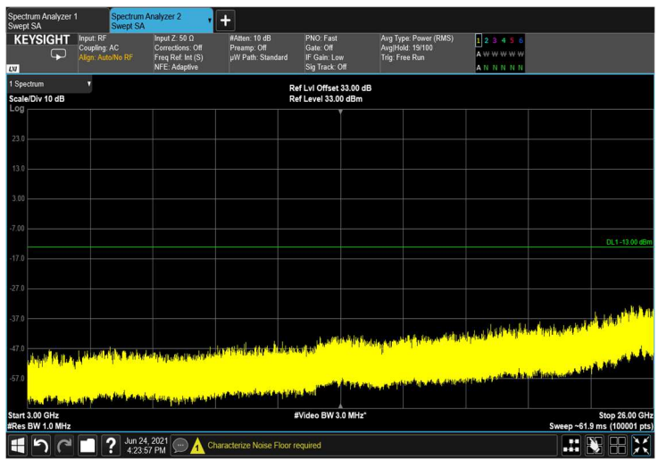
Figure 397: 3GHz-26GHz
