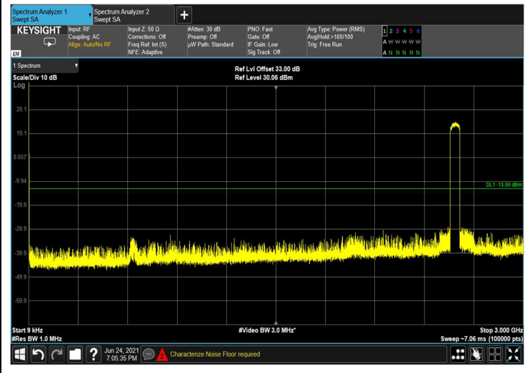
Figure 414: 9kHz-3GHz
