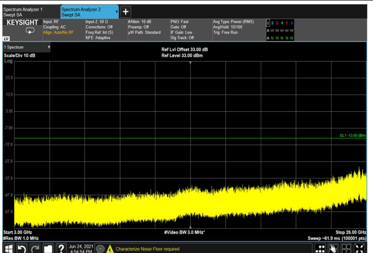
Figure 395: 3GHz-26GHz
