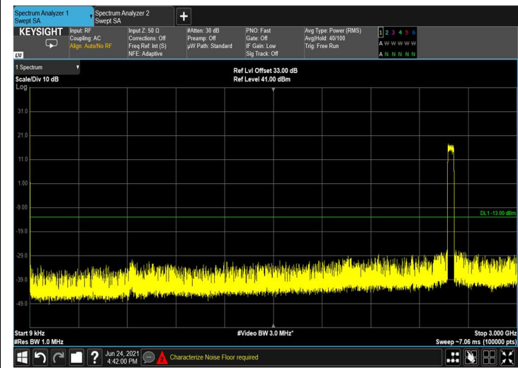
Spurious Emissions at Antenna Terminal QPSK 40MHz B.W.; 2593.0MHz, 30kHz
