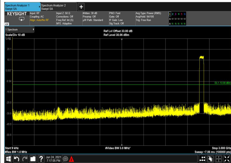
Figure 410: 9kHz-3GHz
