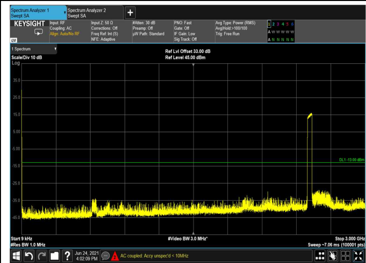
Figure 420: 9kHz-3GHz
