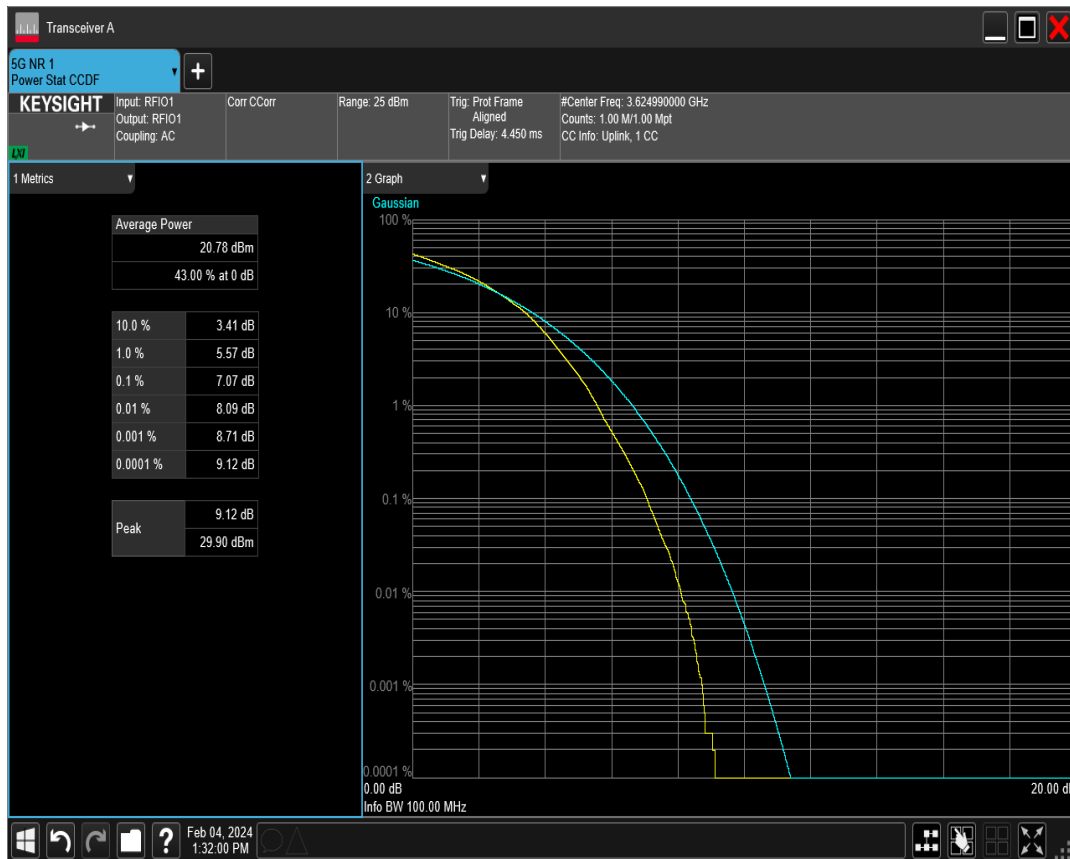
n77(3550-3700) SCS=30kHz DFT_BPSK BW=90MHz Channel=641666 RB=240@0
