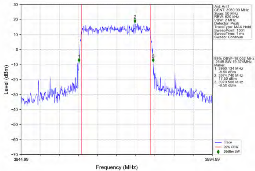
n77a_30kHz_SISO_NTNV_20MHz_DFT-s-OFDM_QPSK_3969.99MHz_Outer_Full
