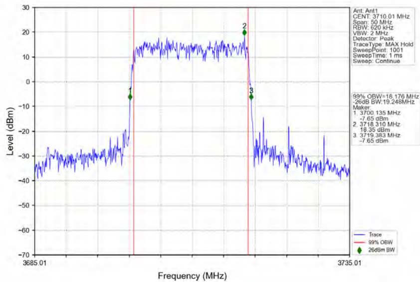
n77a_30kHz_SISO_NTNV_20MHz_DFT-s-OFDM QPSK 3710.01MHz_Outer_Full
