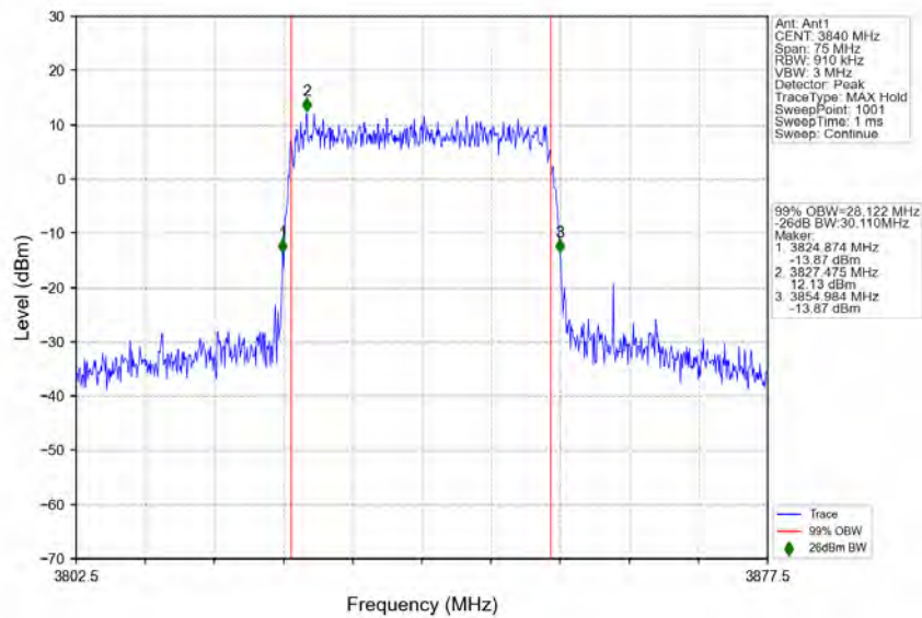
n77a 30kHz SISO NTN 30MHz CP-OFDM 256 QAM 3840MHz Outer Full
