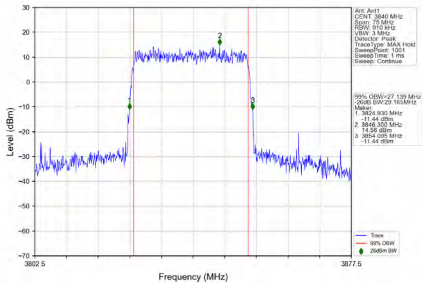
n77a 30kHz SISO NTN 30MHz DFT-s-OFDM 256 QAM 3840MHz Outer Full
