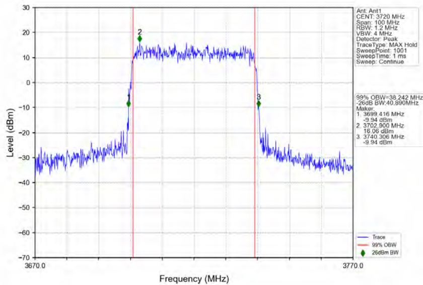
n77a_30kHz_SISO_NTNV_40MHz_CP-OFDM_64_QAM_3720MHz_Outer_Full
