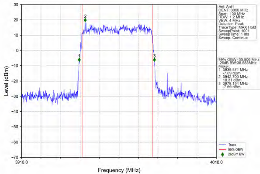
n77a 30kHz SISO NTN 40MHz DFT-s-OFDM QPSK 3960MHz Outer Full
