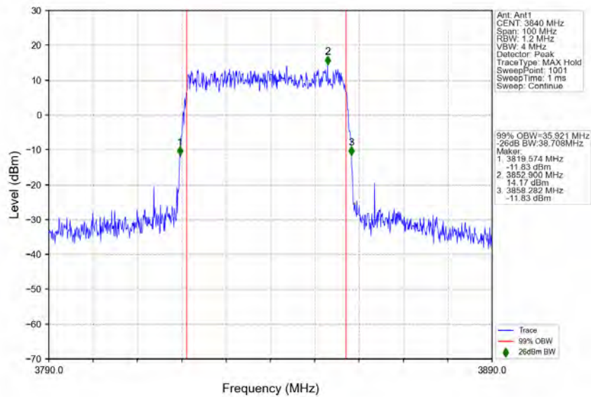
n77a 30kHz SISO NTN 40MHz DFT-s-OFDM 256 QAM 3840MHz Outer Full
