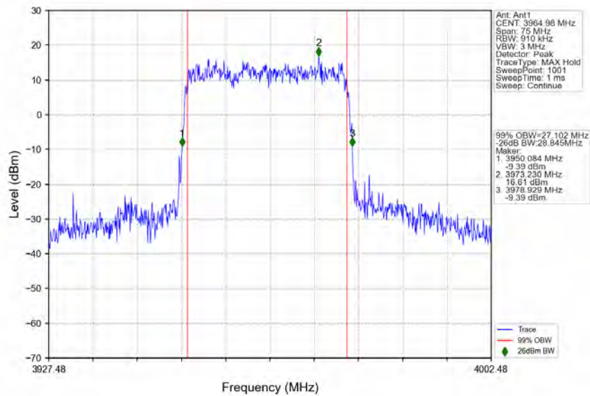
n77a_30kHz_SISO_NTNV_30MHz_DFT-s-OFDM_64_QAM_3964.98MHz_Outer_Full
