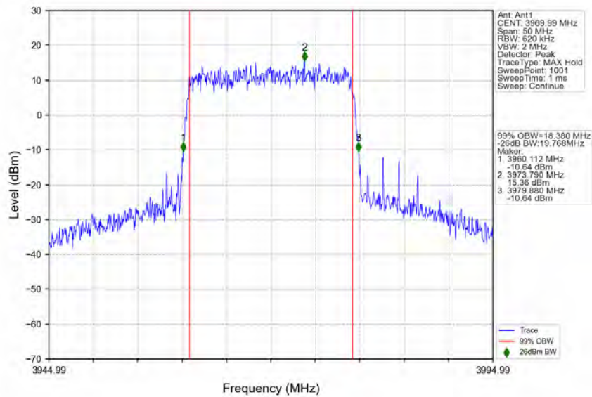
n77a_30kHz_SISO_NTNV_20MHz_CP-OFDM_64_QAM_3969.99MHz_Outer_Full
