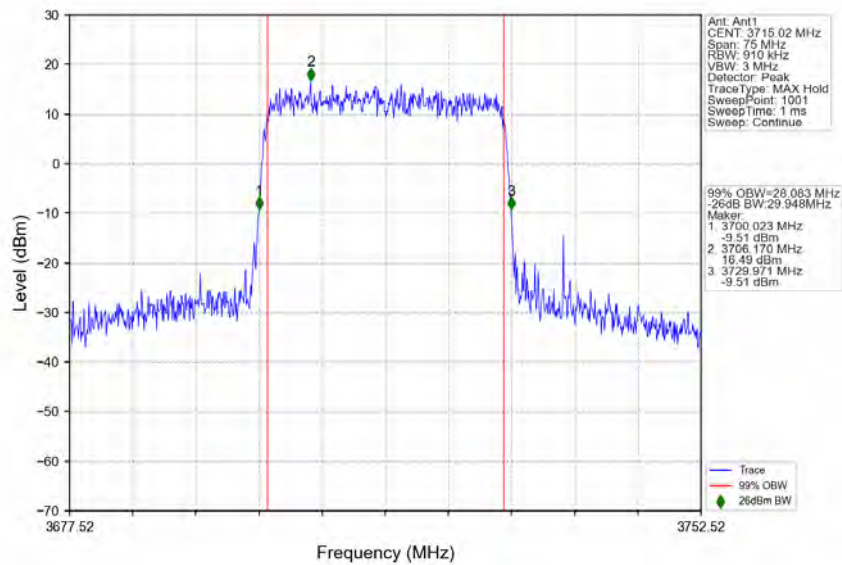
n77a_30kHz_SISO_NTNV_30MHz_CP-OFDM_QPSK_3715.02MHz_Outer_Full
