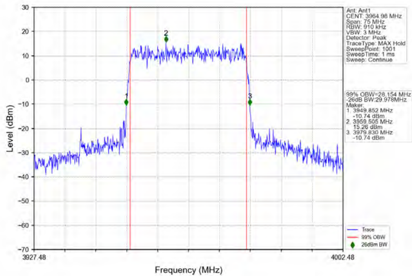
n77a_30kHz_SISO_NTNV_30MHz_CP-OFDM_64_QAM_3964.98MHz_Outer_Full
