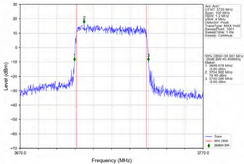
n77a 30kHz SISO NTN 40MHz CP-OFDM QPSK 3720MHz Outer Full
