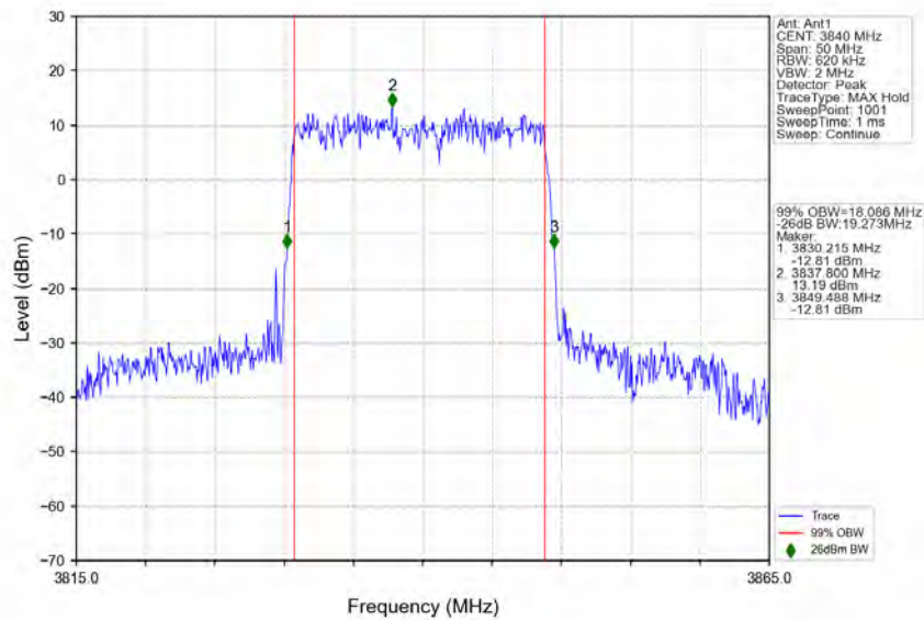
n77a 30kHz SISO NTN 20MHz DFT-s-OFDM 256 QAM 3840MHz Outer Full
