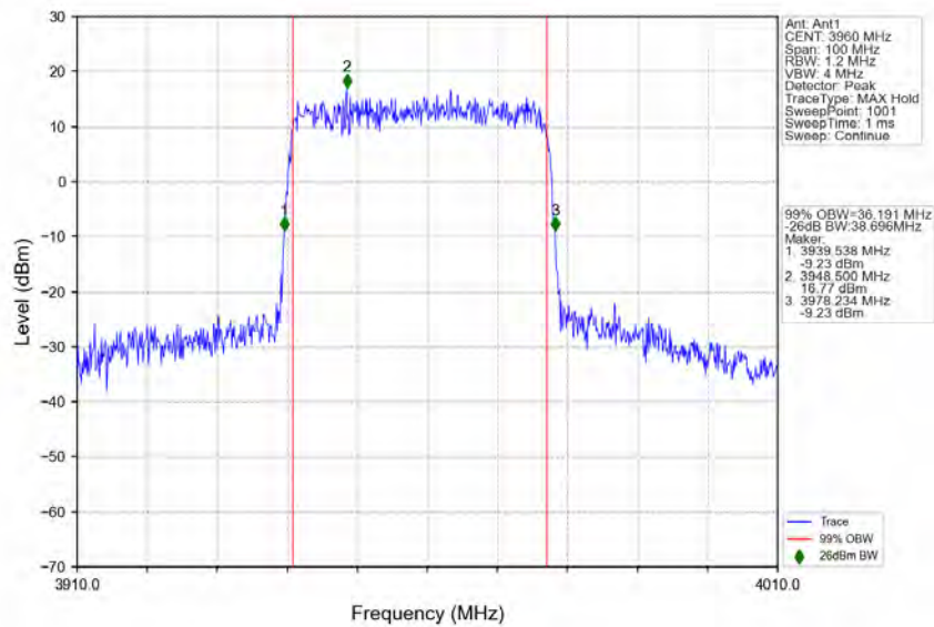
n77a_30kHz_SISO_NTNV_40MHz_DFT-s-OFDM_64_QAM_3960MHz_Outer_Full
