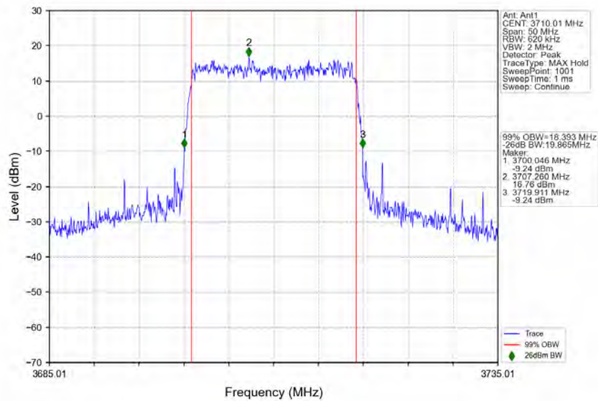
n77a 30kHz SISO NTN 20MHz CP-OFDM QPSK 3710.01MHz Outer Full
