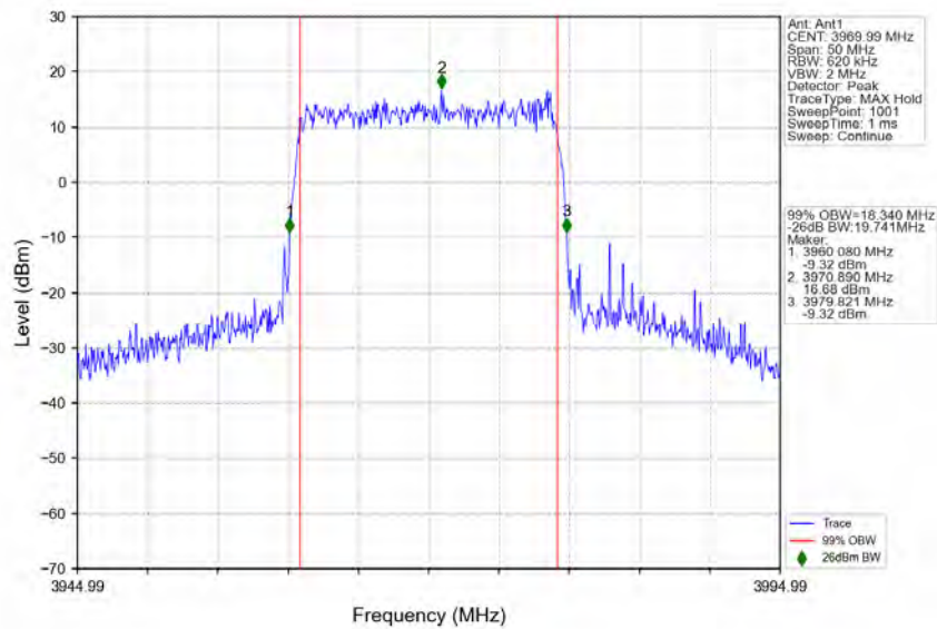
n77a_30kHz_SISO_NTNV_20MHz_CP-OFDM_QPSK_3969.99MHz_Outer_Full
