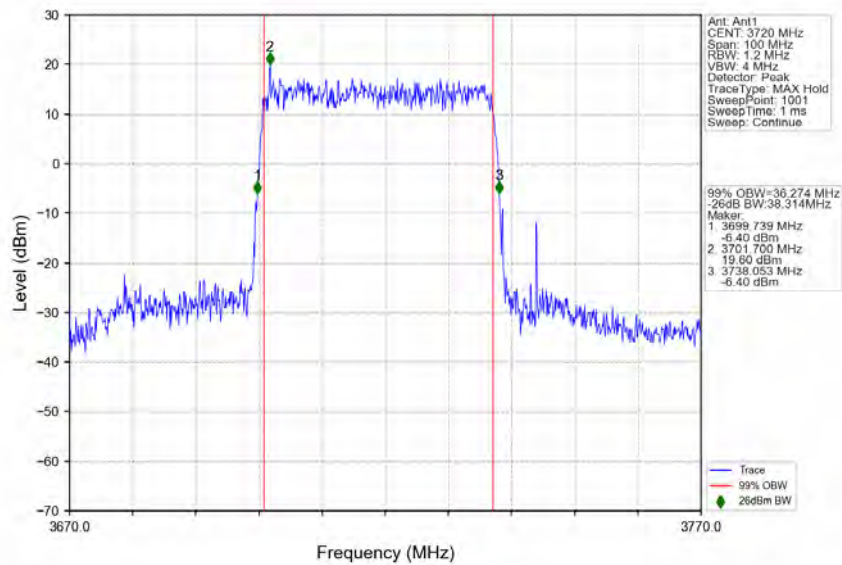
n77a_30kHz_SISO_NTNV_40MHz_DFT-s-OFDM_QPSK_3720MHz_Outer_Full
