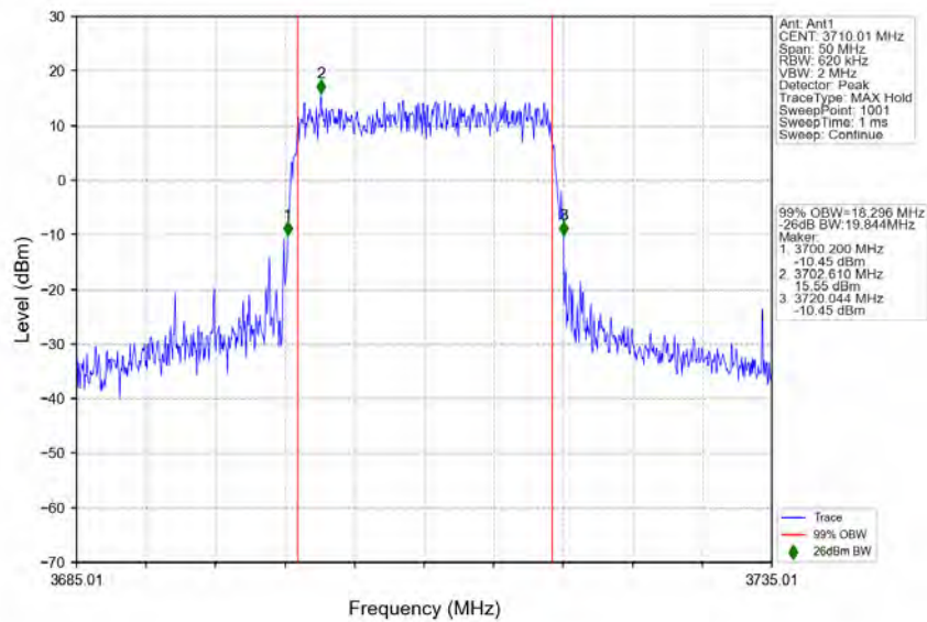
n77a_30kHz_SISO_NTNV_20MHz_CP-OFDM_64_QAM_3710.01MHz_Outer_Full
