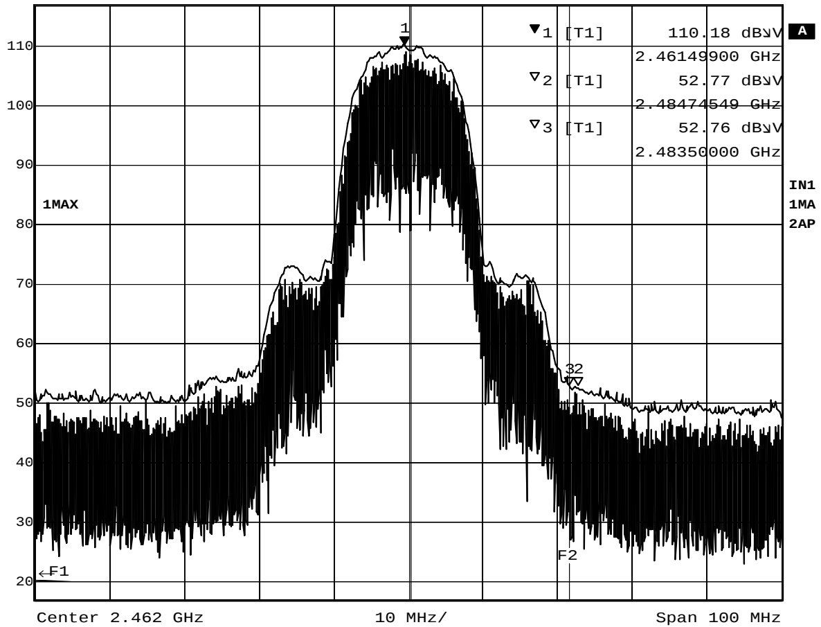
Plot 8-3 Ch.11 2462MHz TX, 11Mbps (Peak)
