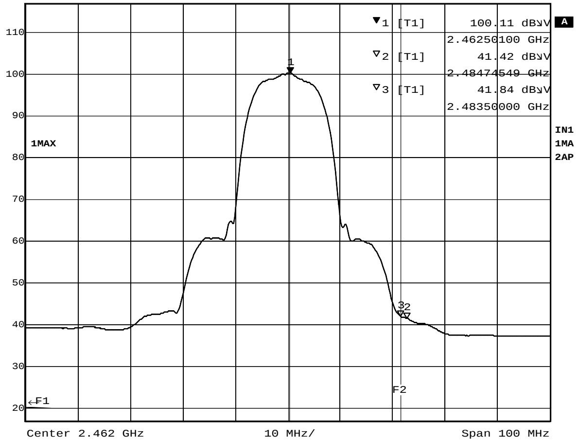
Plot 8-4 Ch.11 2462MHz TX, 11Mbps (Average)
