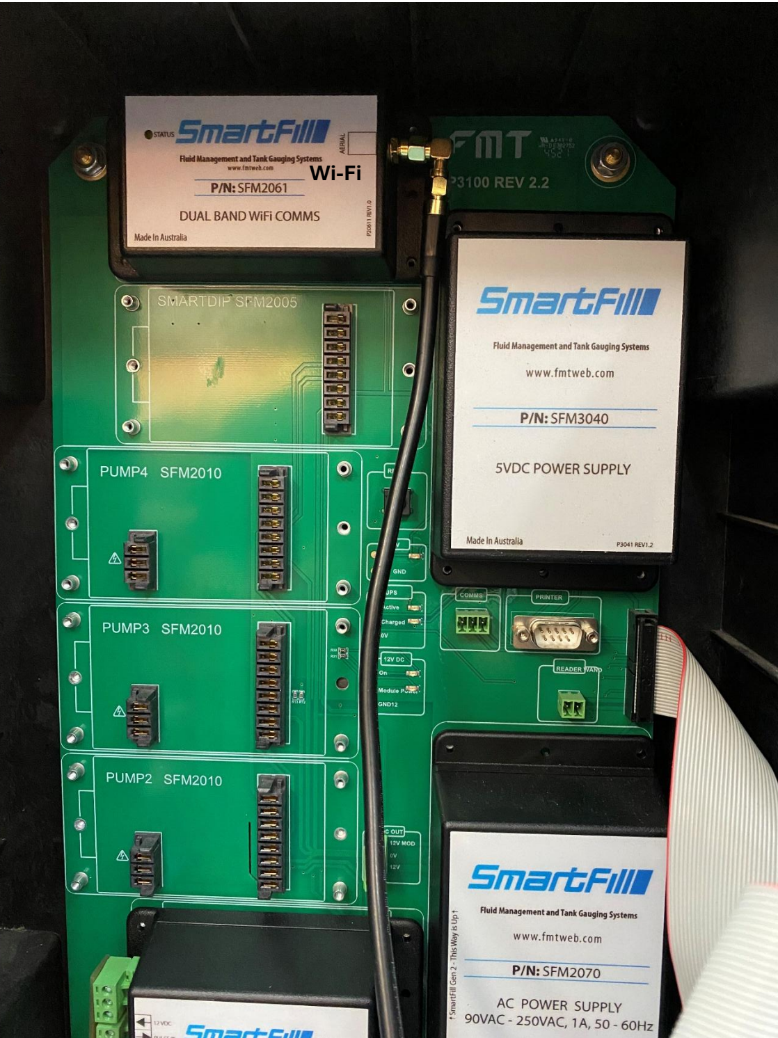
Internal picture with Wi-Fi module:
