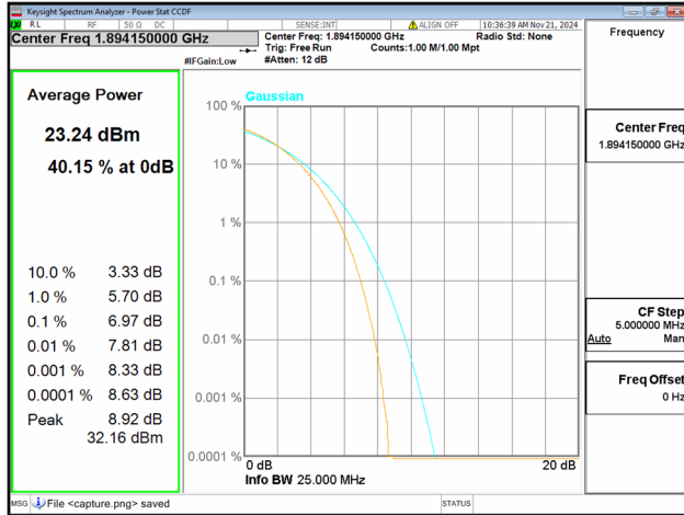
2C / 5+20MHz / High CH / 64QAM
