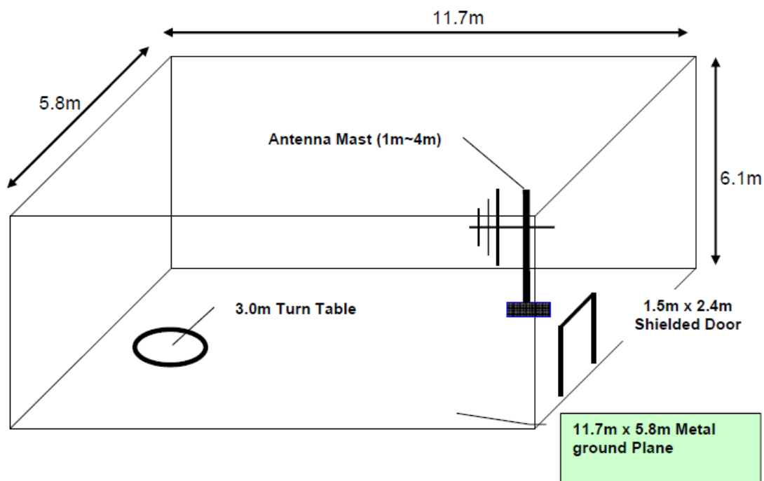
FIGURE 3 - LAYOUT OF 5 METER SEMI-ANECCHOIC CHAMBER
