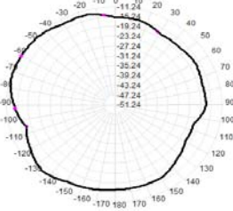
Total(H-XY), Max=-12.19dB, CrD=9.72
