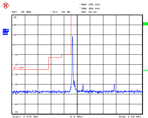
LTE Band 7 QPSK 10MHz CH-Low, 1 RB
