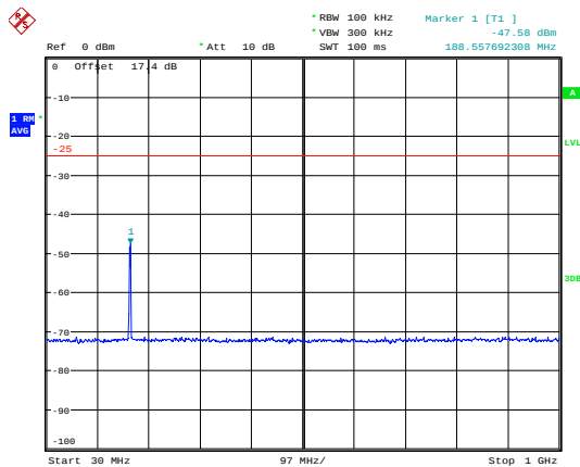
LTE Band 7 5MHz CH-Low 30MHz~1GHz
