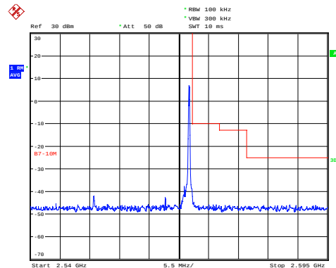
LTE Band 7 QPSK 10MHz CH-High, 1 RB
